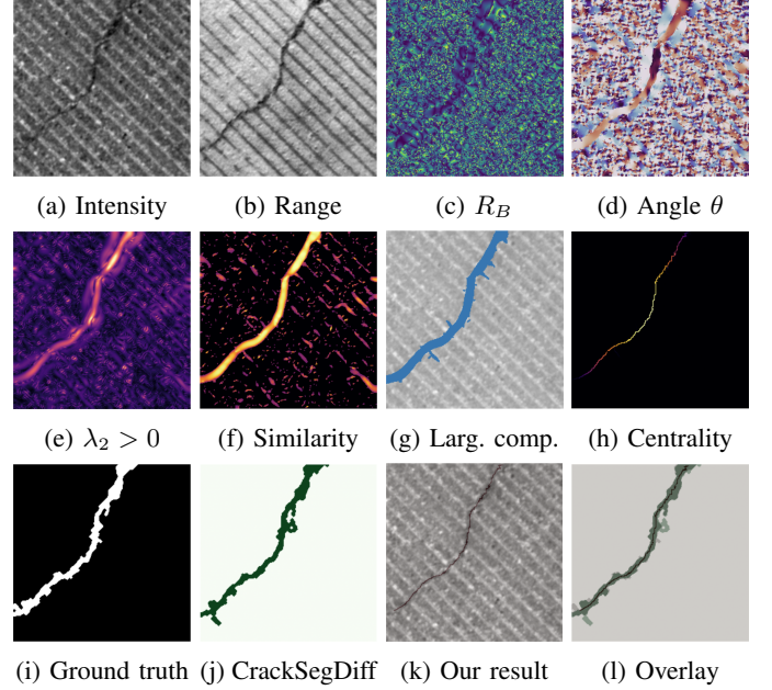
Fig. 2: Processing of the first FIND image example. Top row: (a) Top: Intensity and (b), Range modalities, (c) FRANGI ratio R_B = |\lambda_1|/|\lambda_2| and (d) map of \sin(\theta) associated to the Hessian orientation. Middle row: (e) Map x \mapsto \lambda_2 \mathbf{1}_{\lambda_2 > 0} (very close to the original FRANGI filter) Middle: Positive curvature, (f) Our FRANGI similarity ( x_i \mapsto \max_{j, x_i \sim x_j} S_{ij} ), (g) the largest cluster component and (h) the weighted betweenness-centrality. Bottom row: (i) Bottom: Ground truth, (j) Result of CrackSegDiff on fused modalities, ours (k) Our resulting skeleton (JACCARD / IoU: 63% ; TVERSKY: JACCARD, 71% ; WASSERSTEIN: TVERSKY, 8px WASSERSTEIN) and (l) Overlay of ground truth, CrackSegDiff and our skeleton overlay.
