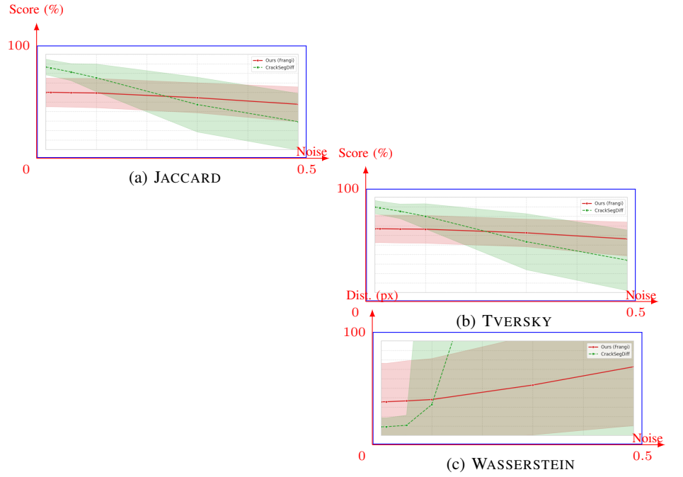
Fig. 4: Performance degradation on noisy FIND. Red: Proposed method; green Green: CrackSegDiff. Shaded regions show standard deviation. The horizontal axis is the noise level s (standard deviation of the Gaussians).
