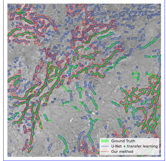
Fig. 6: Qualitative comparison on the Test2 Vaches Noires image (France) Test2 . The ground Ground truths shown in green , our method in red, and Green ; Ours: Red; U-Net + transfer learning in blue : Blue.
