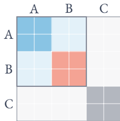
Foundation-model attention
