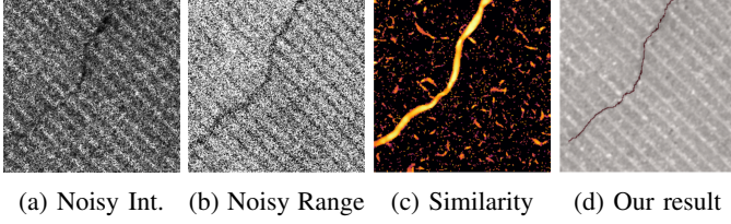
Fig. 4: Noisy FIND example ( s = 0.5 ) with speckle noise on intensity and Gaussian noise on range. The graph similarity remains concentrated around the main crack.
