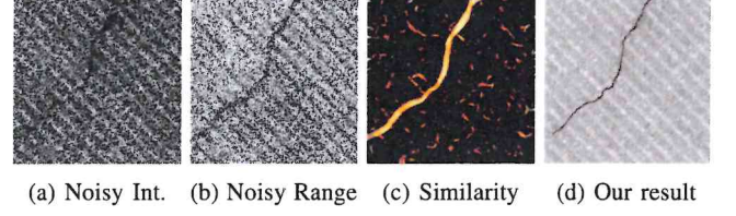
Fig. 3: Noisy FIND example ( s = 0.5 ) with speckle noise on intensity and Gaussian noise on range. The graph similarity remains concentrated around the main crack.
