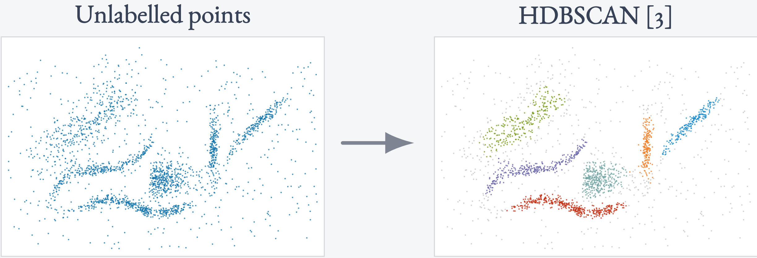
Clusters in colour; unassigned points in grey [3].
