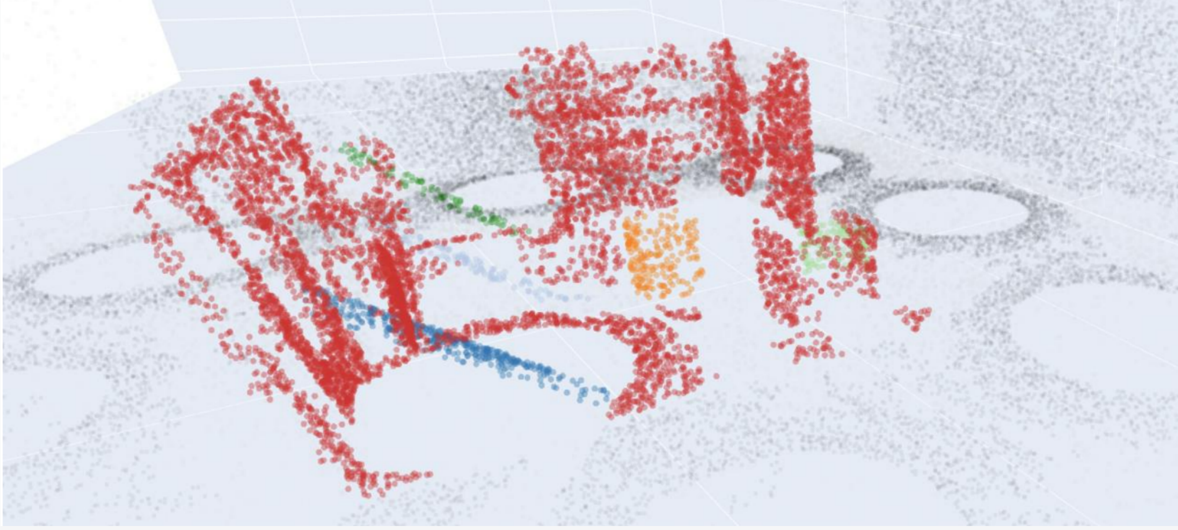
Synthetic benchmark: 2 million points. Red: model-consistent; other colours: anomalies; grey: background. © Naval Group [6].
