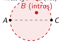
Non-Gabriel (non vide)
