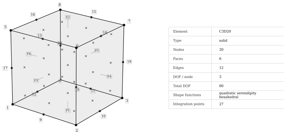
Figure 6.7: C3D20 quadratic hexahedral solid element.
