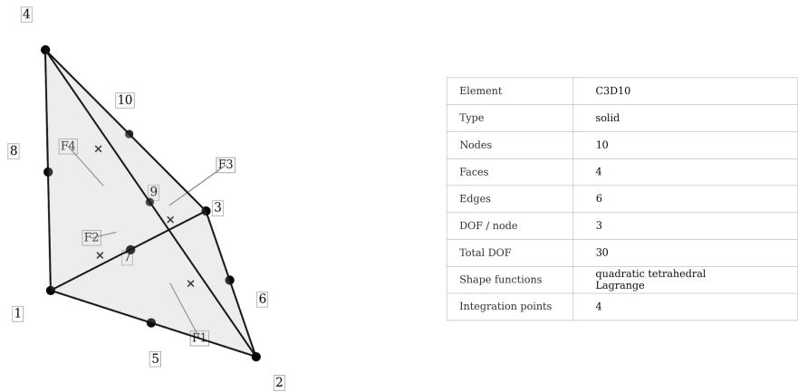
Figure 6.4: C3D10 quadratic tetrahedral element.
