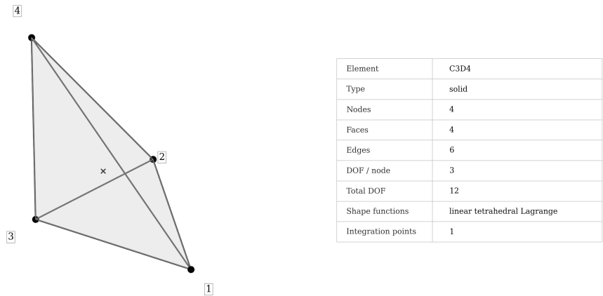
Figure 5.1: C3D4 element topology and integration scheme.
