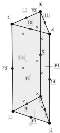
Figure 6.6: C3D15 quadratic wedge element.
