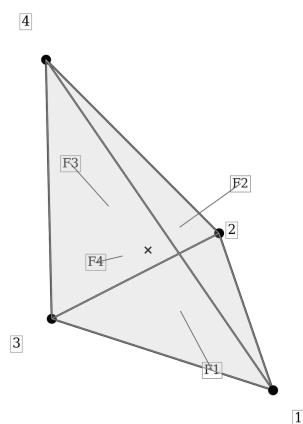
Figure 6.1: C3D4 element topology and integration scheme.
