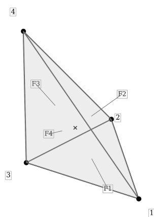
Figure 6.1: C3D4 element topology and integration scheme.
