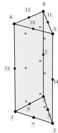
Figure 5.7: C3D15 quadratic wedge element.
