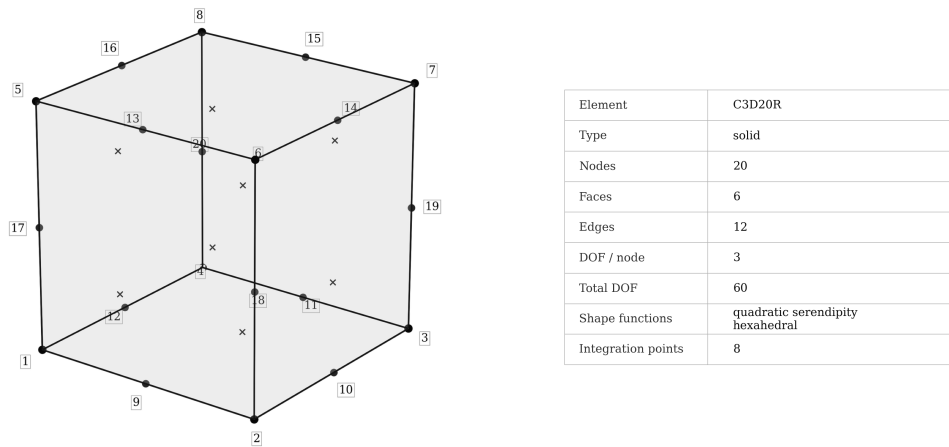
Figure 5.9: C3D20R reduced-integration quadratic hexahedral solid element.
