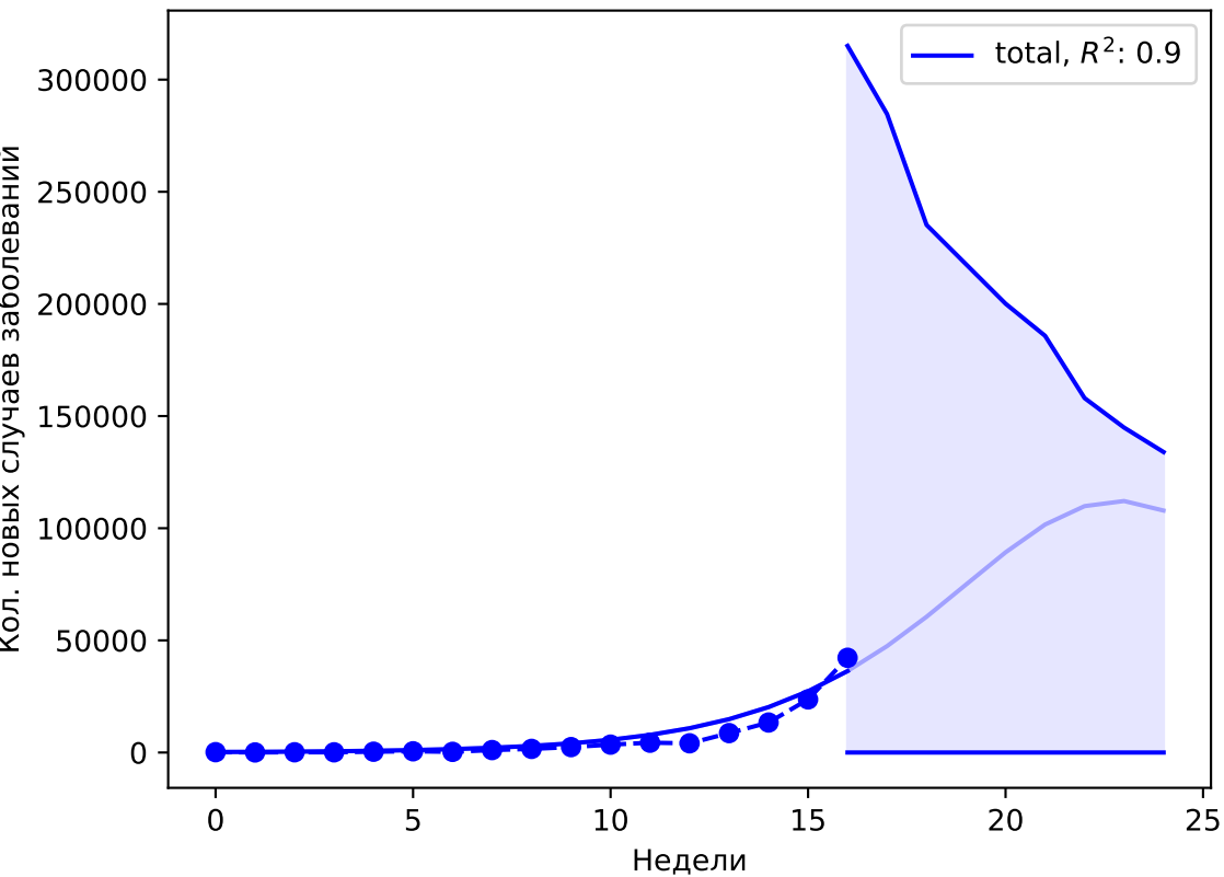
MCMC, Total
