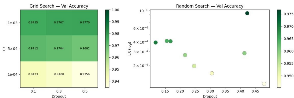
Figure 5 : Grid Search et Random Search - Val Accuracy
