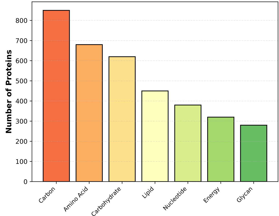
A) Top KEGG Pathways
