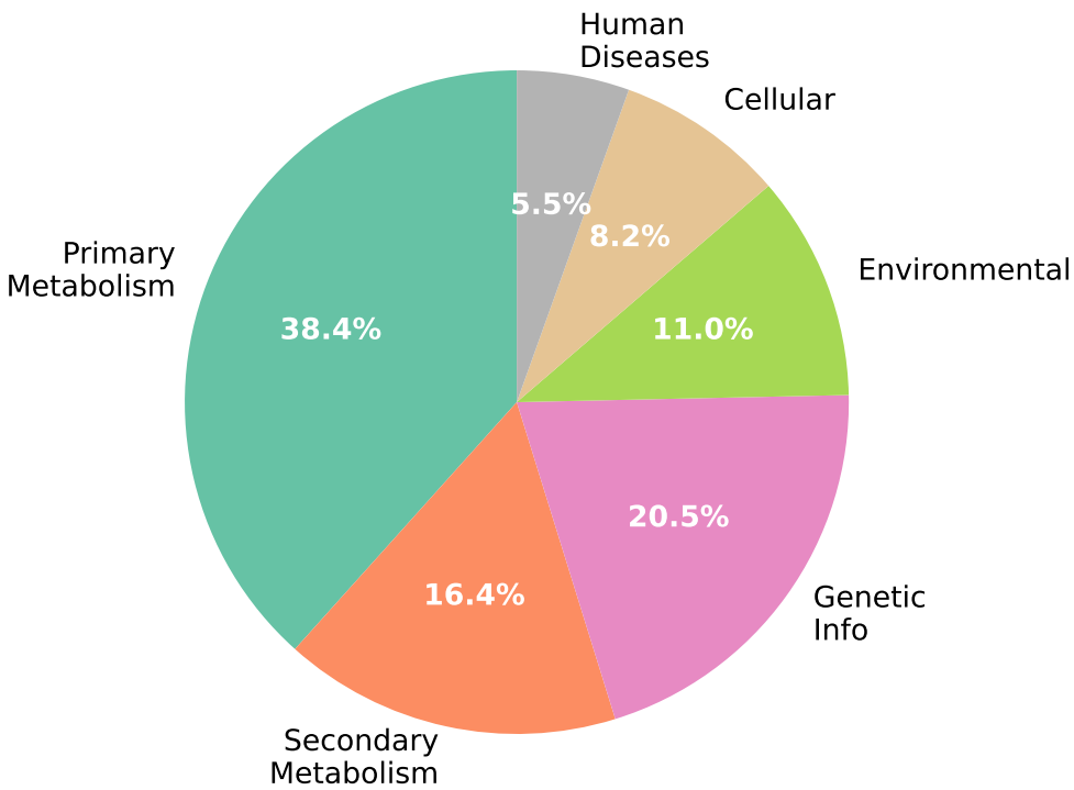
B) KEGG Metabolic Categories
