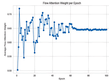
(b) GA-GNN
