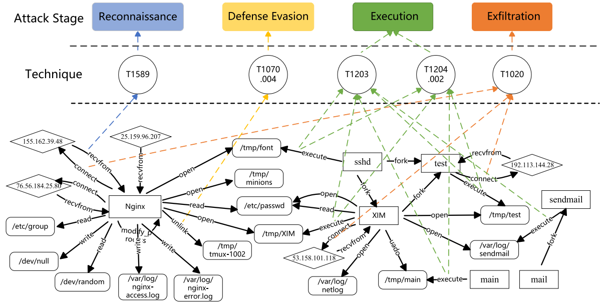
Fig. 6. Attack scenario from Nginx backdoor w/ Drakon in-memory.
