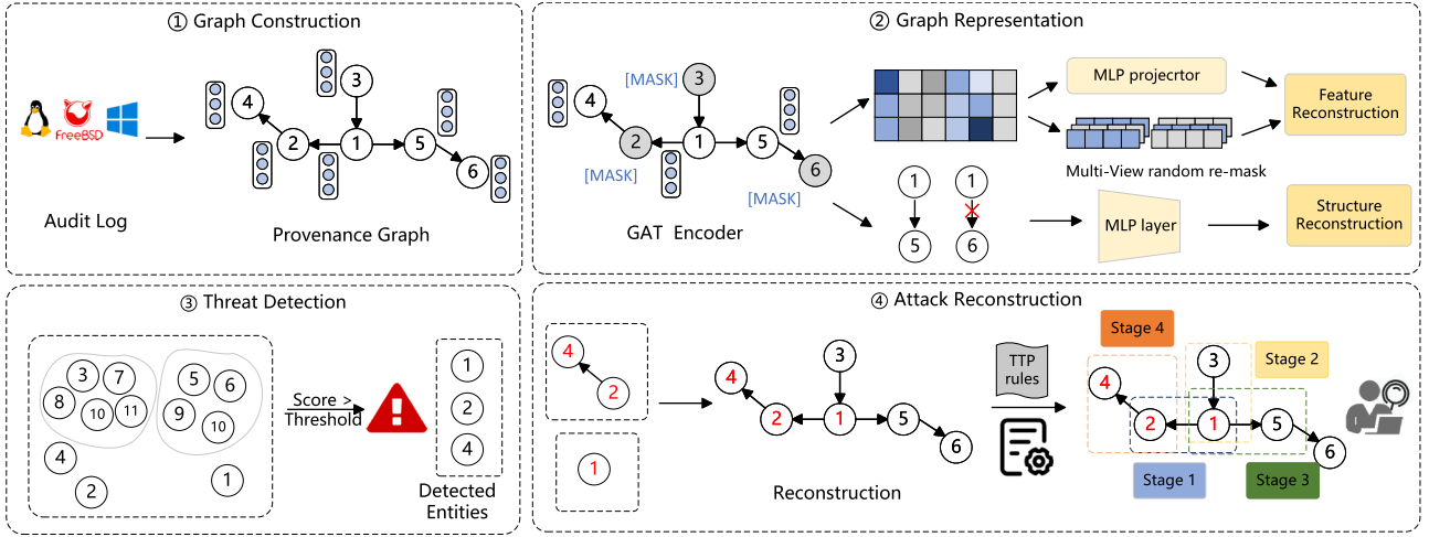
Fig. 2. The framework of MGDA.
