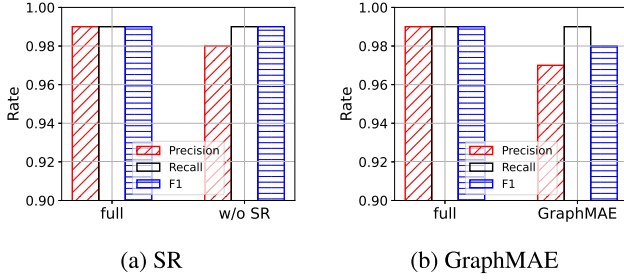
Fig. 5. Ablation study.
