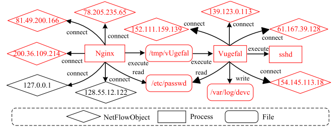
Fig. 1. Attack scenario from DARPA E3 CADETS.
