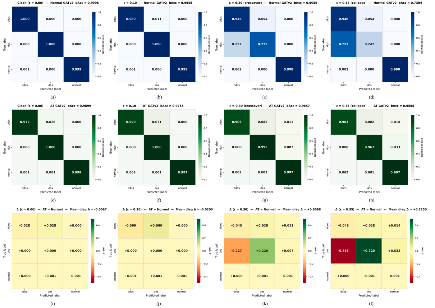
Fig. 4. Normalised confusion matrices for normal (a)–(d) and AT (e)–(h) GATv2 models across PGD perturbations. Per-cell differences \Delta (i)–(l) highlight performance shifts.
