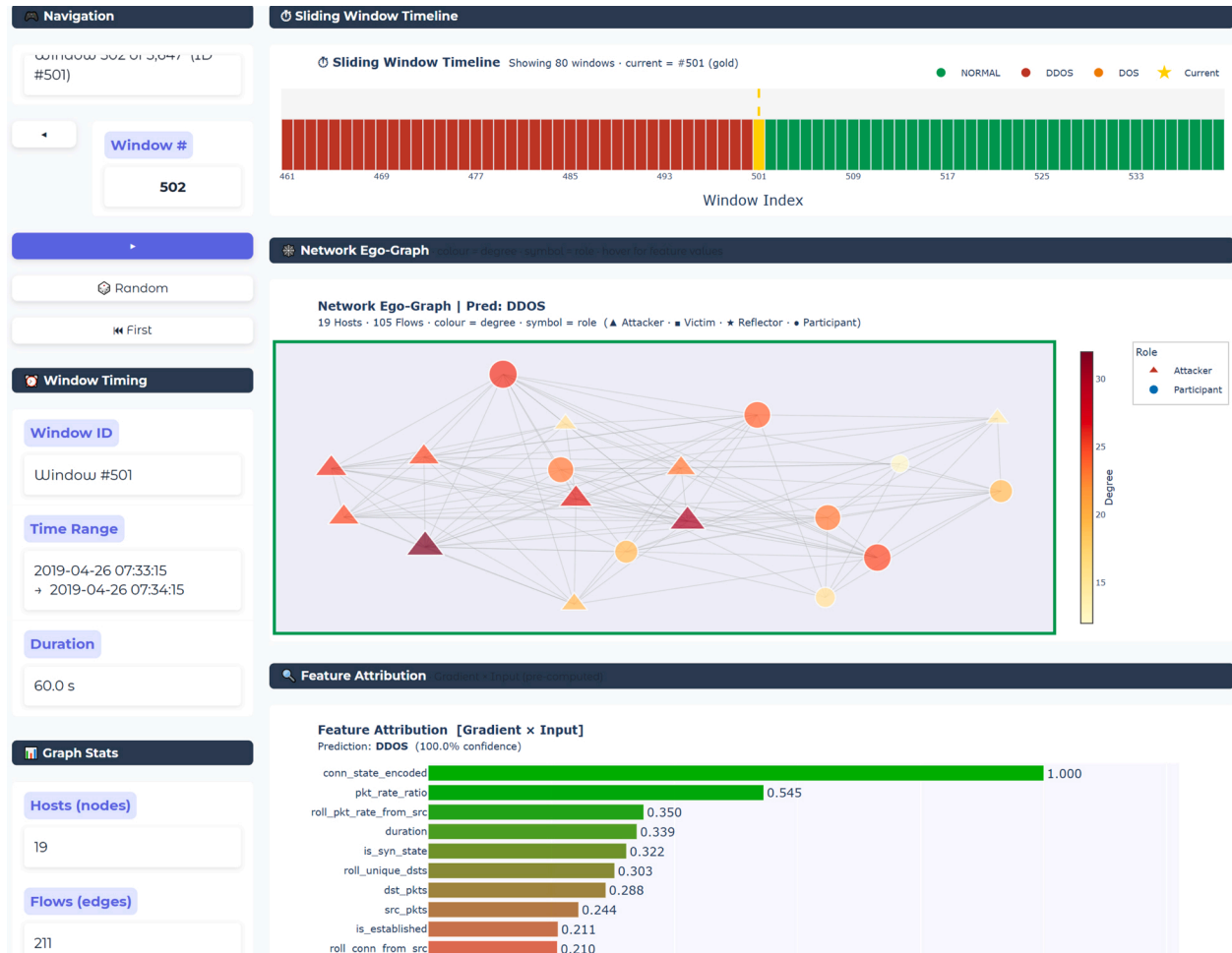
Fig. 7. A gradio dashboard for AT TFA-GATv2 inspection across test graphs, showing timeline, ego-graph, and attribution scores.
