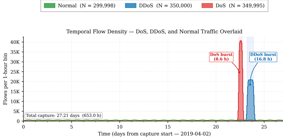
Fig. 2. Temporal flow density of Normal, DoS, and DDoS traffic across 27.21 days capture window.
