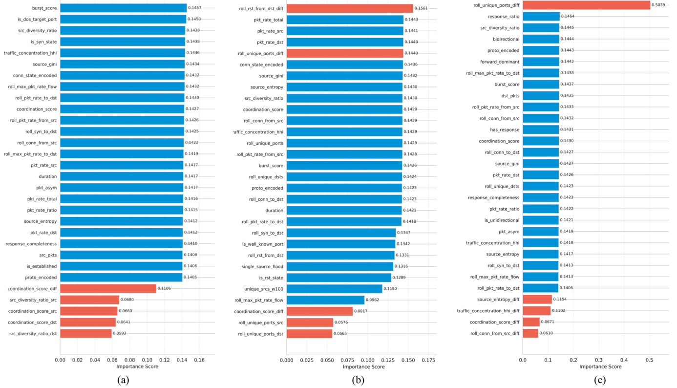
Fig. 5. GNNExplainer top-30 node (blue) and edge (red) feature importances for (a) DDoS, (b) DoS and (c) Normal flow.
