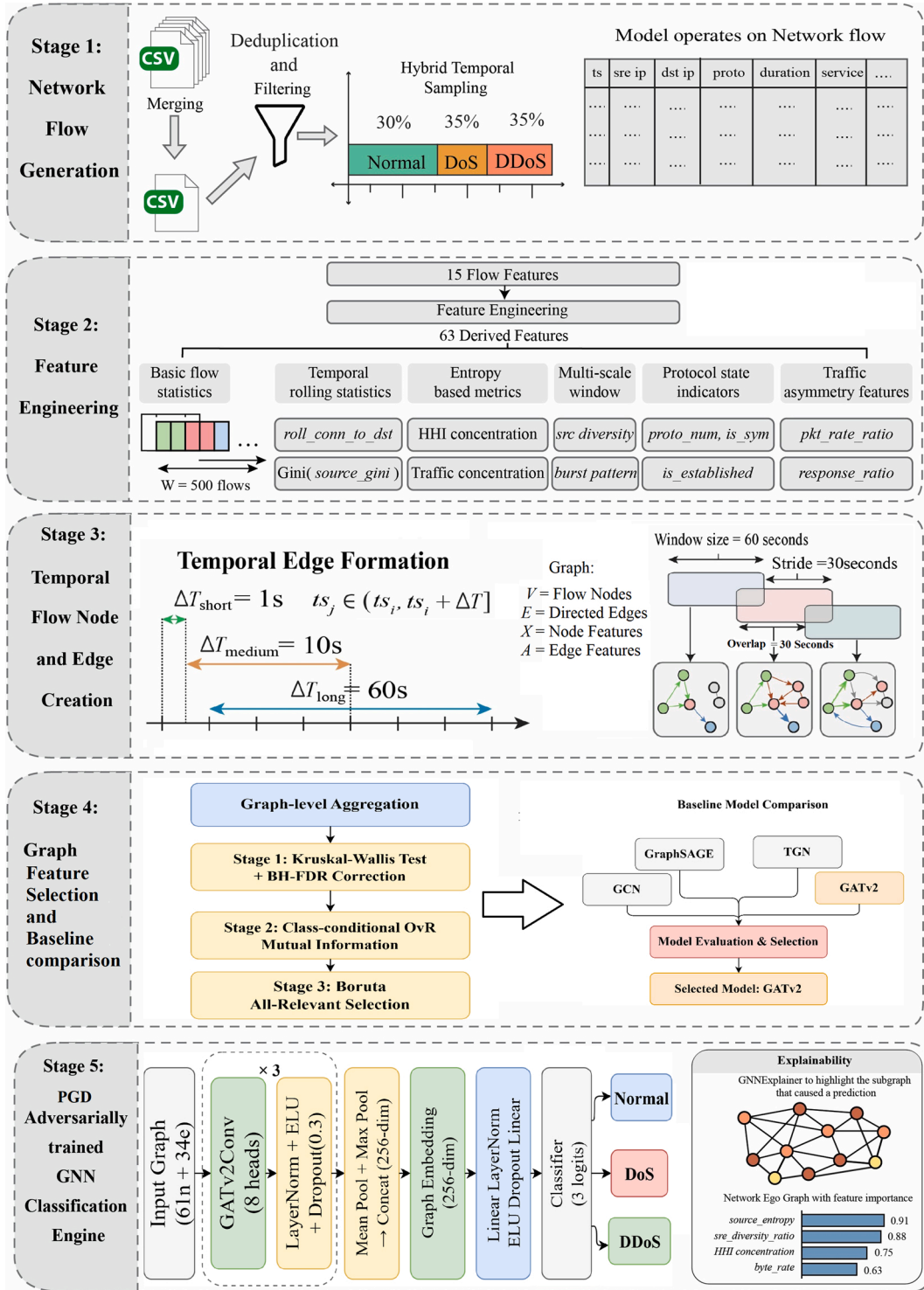
Fig. 1. The Five-stage research workflow with preprocessing, feature engineering, graph constructions, feature selection and PGD-hardened GATv2 model classification.
