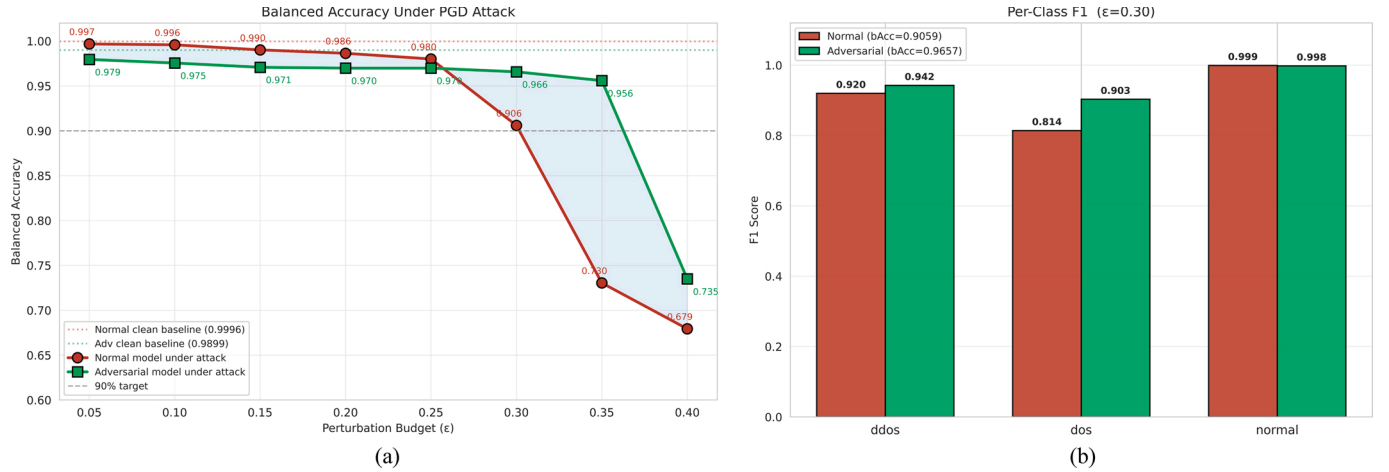
Fig. 3. Comparative analysis of model robustness of Normal vs. AT GATv2 (a) balanced accuracy across \epsilon , and (b) F1 score under adversarial evaluation ( \epsilon = 0.30 ).
