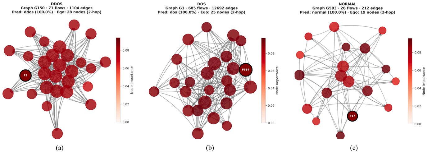
Fig. 6. GNNExplainer Ego-Graph visualization of traffic snapshots of (a) DDoS attack in graph G150, (b) a DoS attack in snapshot graph G1, and (c) normal traffic in graph G503.
