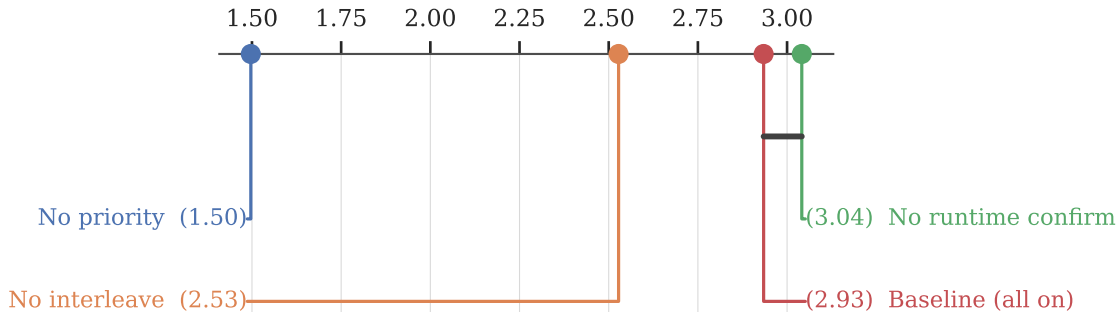
Mean detection-cost rank — Nemenyi post-hoc (n = 776)
