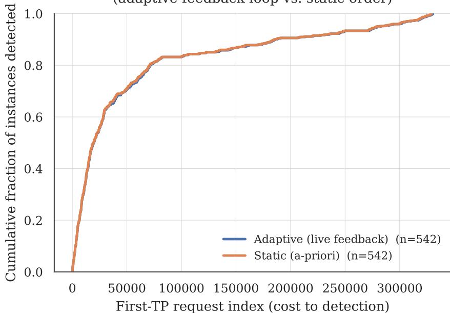
Cost to first true positive (adaptive feedback loop vs. static order)
