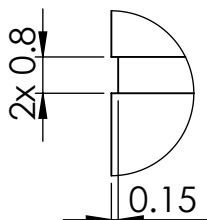
DETAILED ESCALA 6:1
