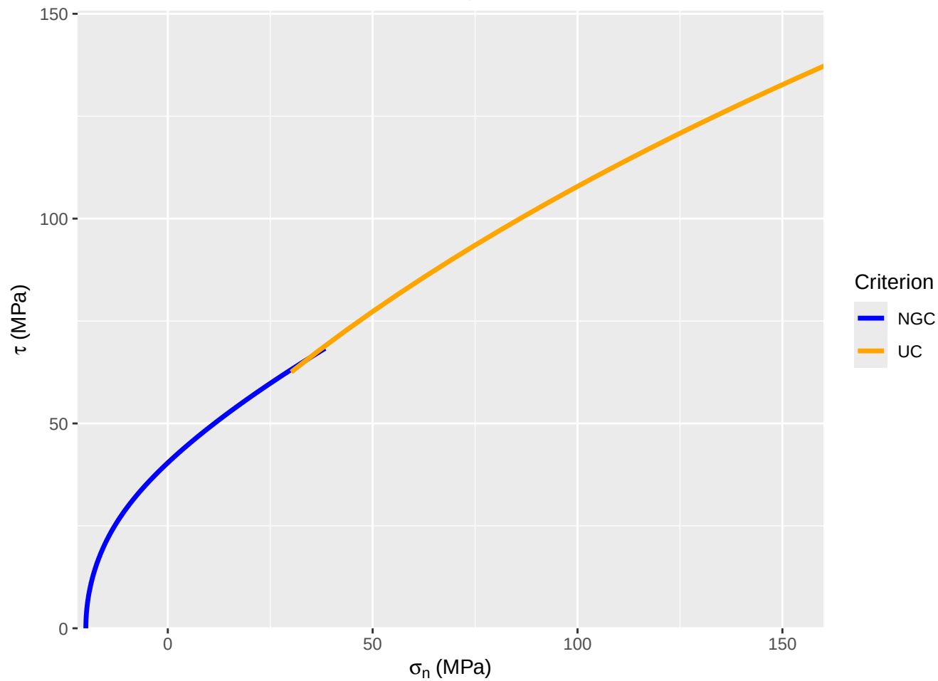
Combined NGC + UC failure envelope
