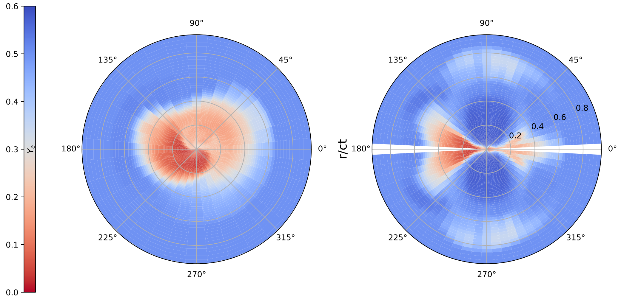
BLh_q1.43 at t = 1016.91 ms
