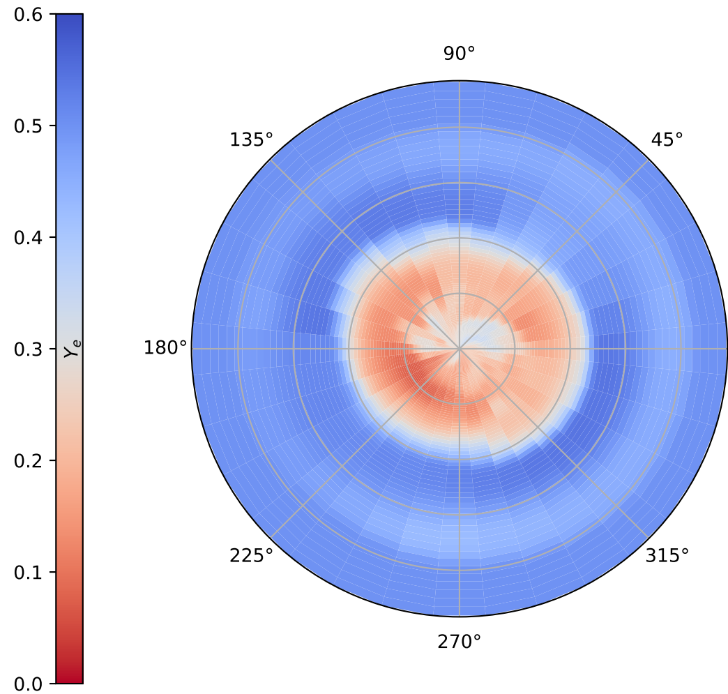
SFHo_q1.0 at t = 1000.05 ms
