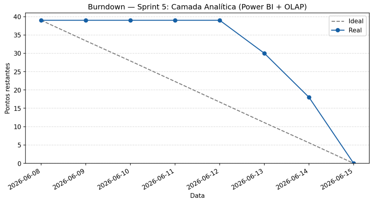
Burndown Sprint 5
