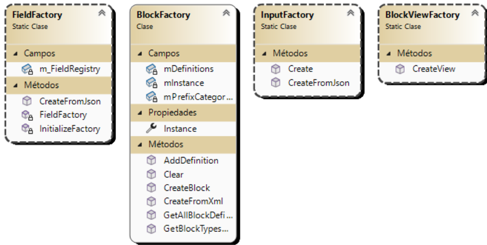
Figura C.9: Diagrama de clases constructores - factory.
