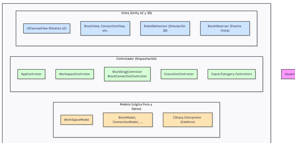
Figura C.1: Diagrama de MVC inicial.
