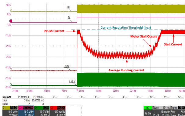
Figure 9-5. Motor startup at 50% duty cycle with current regulation
