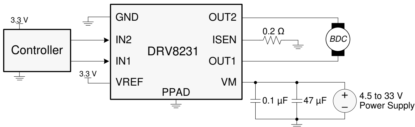
Figure 9-1. Typical Connections
