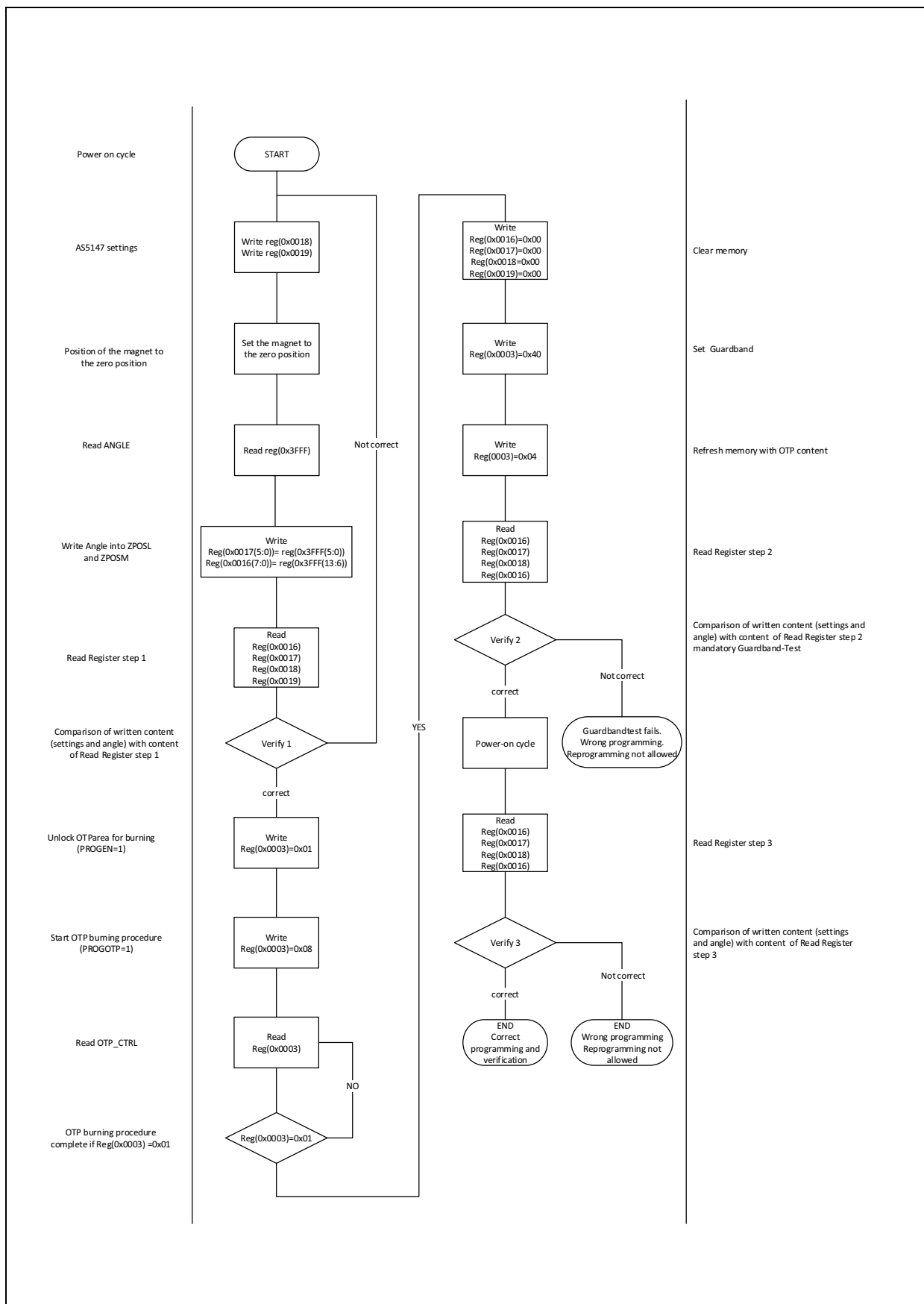
Figure 38: OTP Memory Burn and Verification Flowchart
