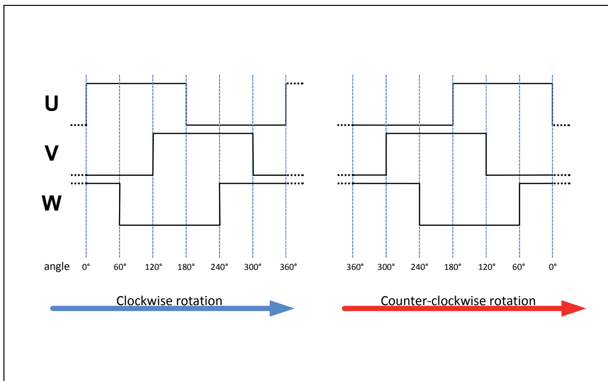
Figure 32: UVW Signals
