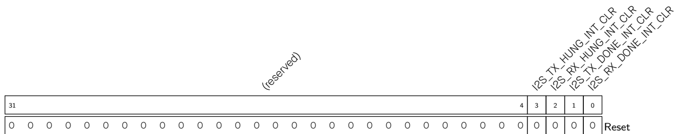
Register 28.4. I2S_INT_CLR_REG (0x0018)
