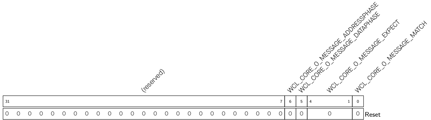
Register 16.5. WCL_CORE_O_MESSAGE_PHASE_REG (0x0108)
