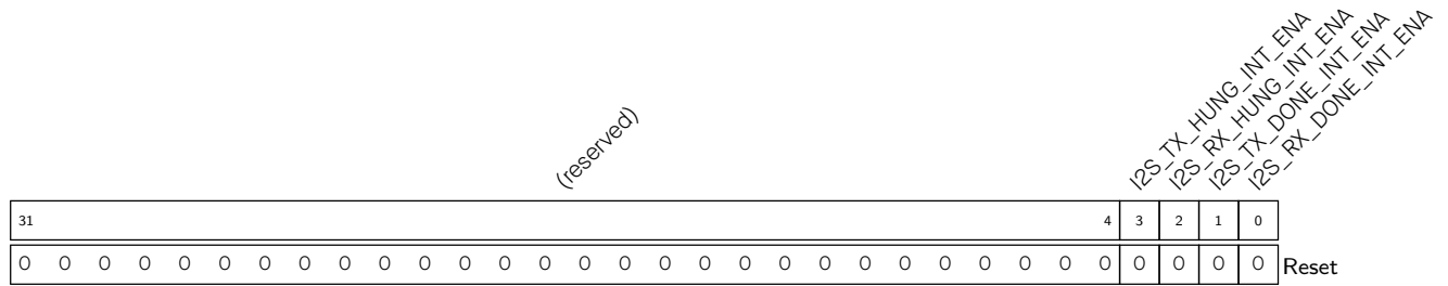
Register 28.3. I2S_INT_ENA_REG (0x0014)
