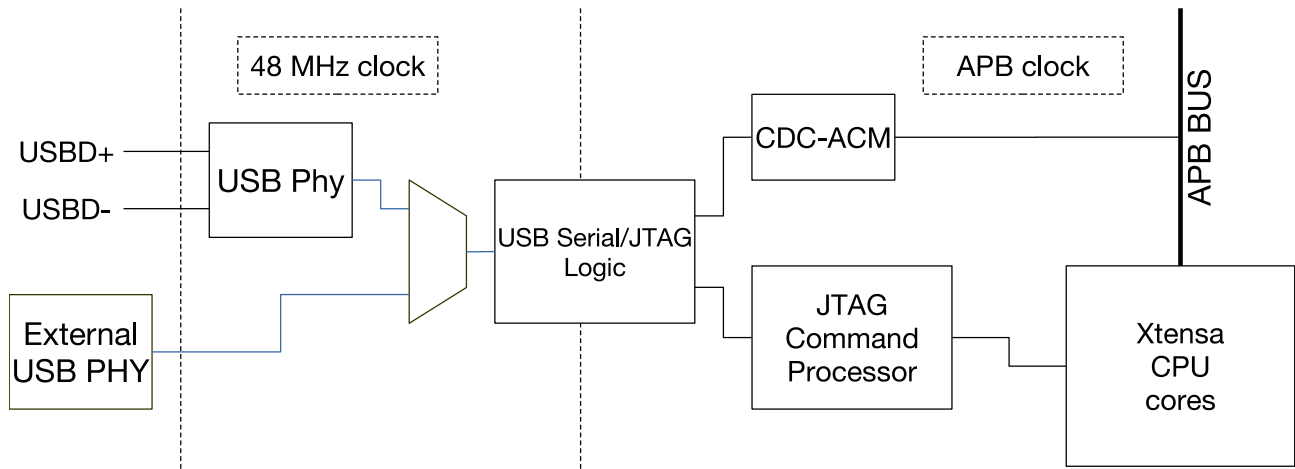
Figure 33.2-1. USB Serial/JTAG High Level Diagram
