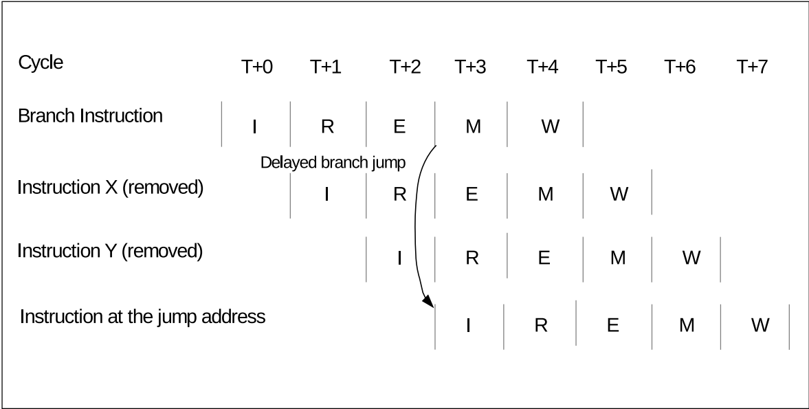
Figure 1.7-3. Control Hazard
