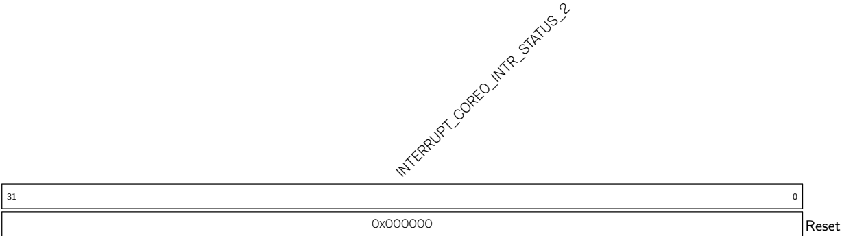
Register 9.87. INTERRUPT_CORE0_INTR_STATUS_2_REG (0x0194)
