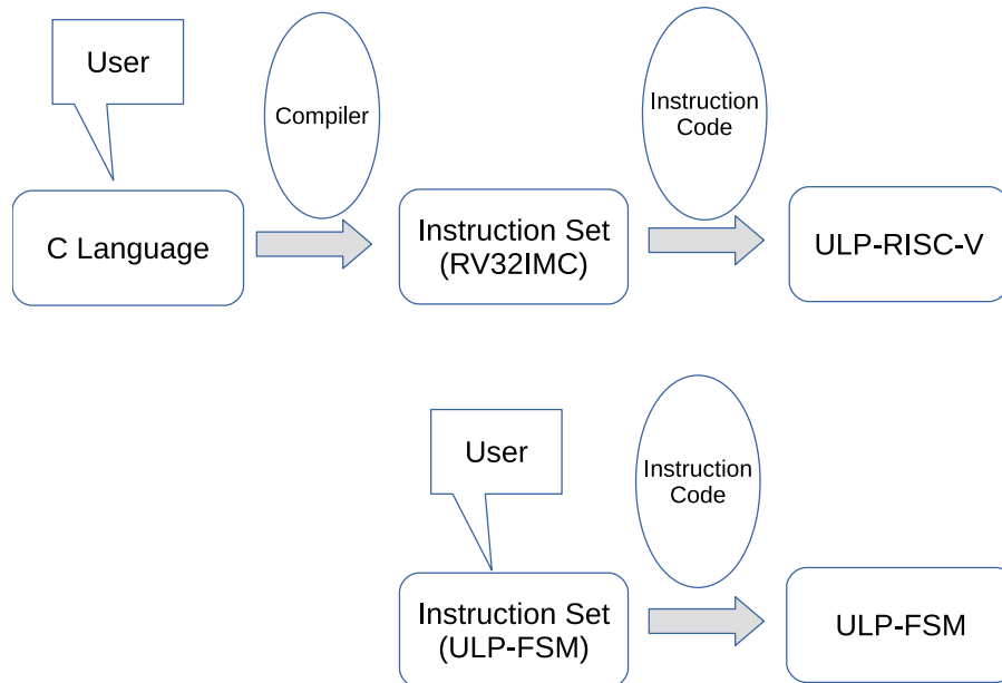
Figure 2.3-1. Programming Workflow
