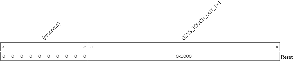
Register 39.22. SENS_SAR_TOUCH_THRES1_REG (0x0064)
