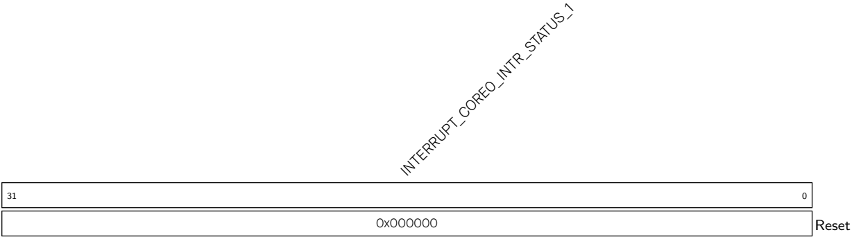
Register 9.86. INTERRUPT_CORE0_INTR_STATUS_1_REG (0x0190)
