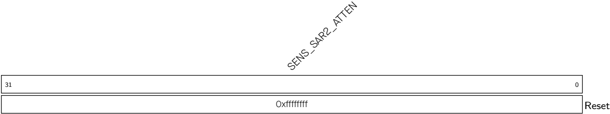
Register 39.17. SENS_SAR_ATTEN2_REG (0x0038)
