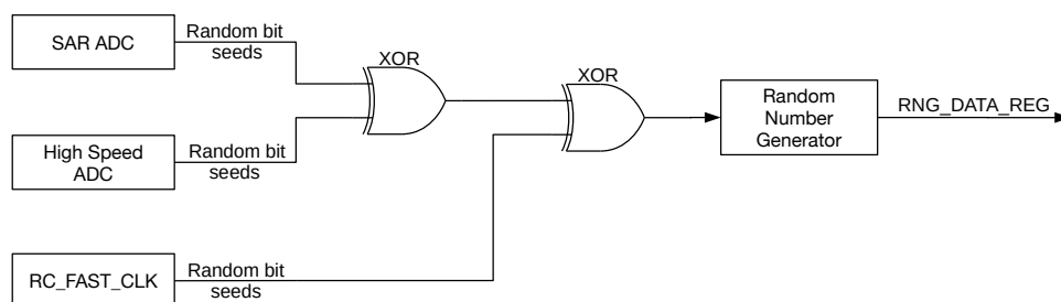
Figure 25.3-1. Noise Source
