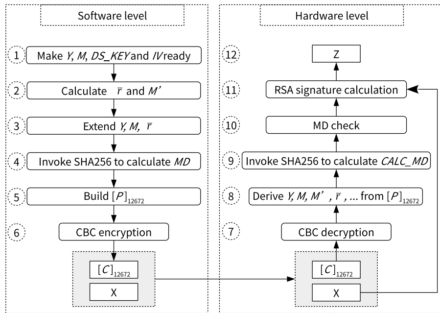
Figure 22.3-1. Software Preparations and Hardware Working Process
