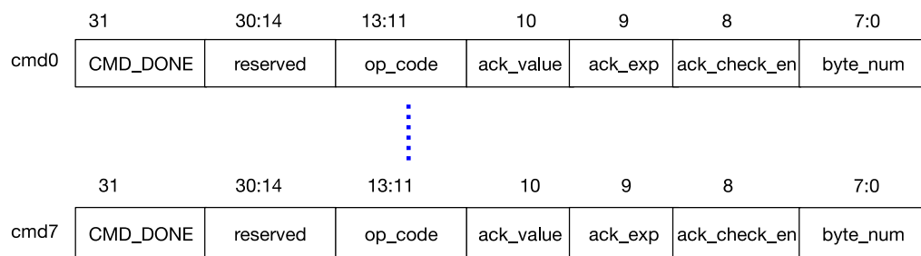
Figure 27.4-2. Structure of I2C Command Registers
