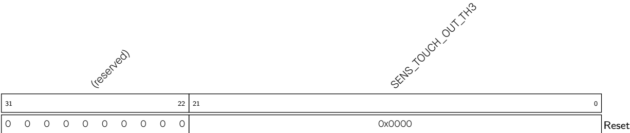
Register 39.24. SENS_SAR_TOUCH_THRES3_REG (0x006C)
