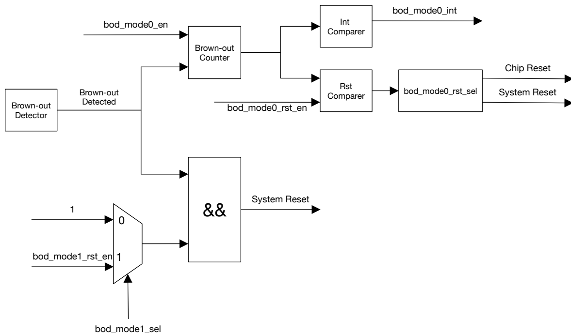
Figure 10.3-9. Brown-out detector
