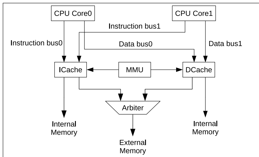
Figure 4.3-1. Cache Structure
