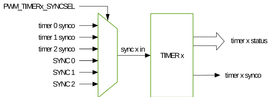
Figure 36.3-2. Timer Submodule
