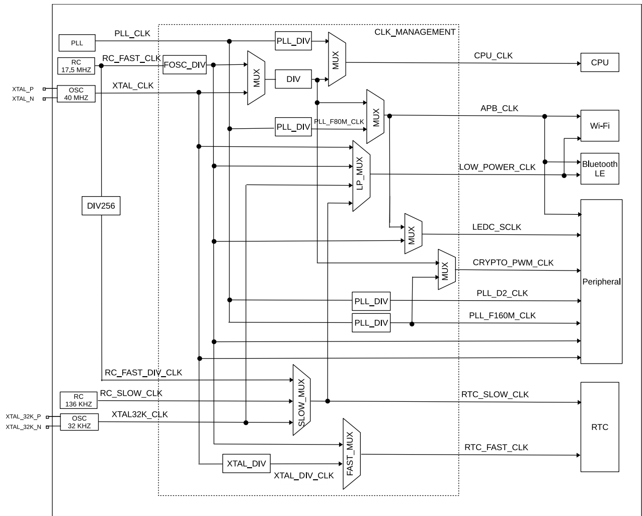
Figure 7.2-1. Clock Structure
