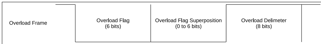
Figure 31.3-3. Fields of an Overload Frame
