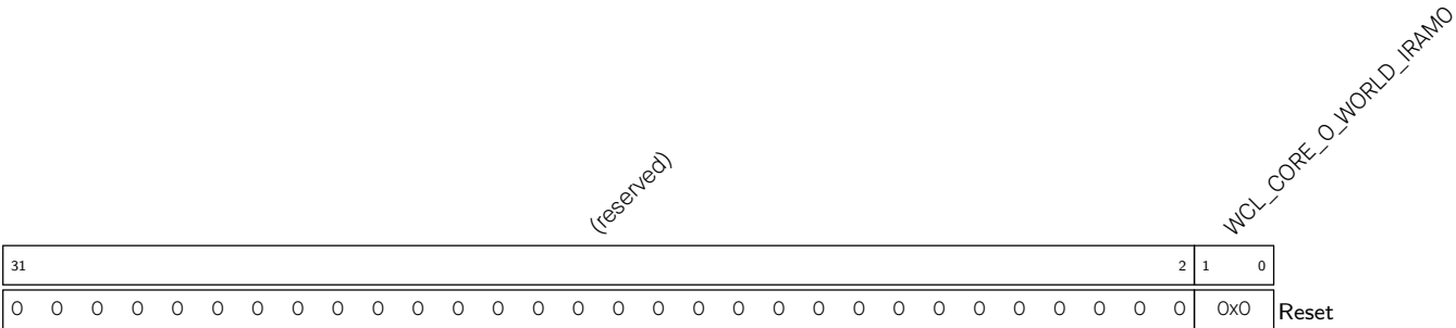
Register 16.12. WCL_CORE_O_World_IRamO_REG (0x0150)
