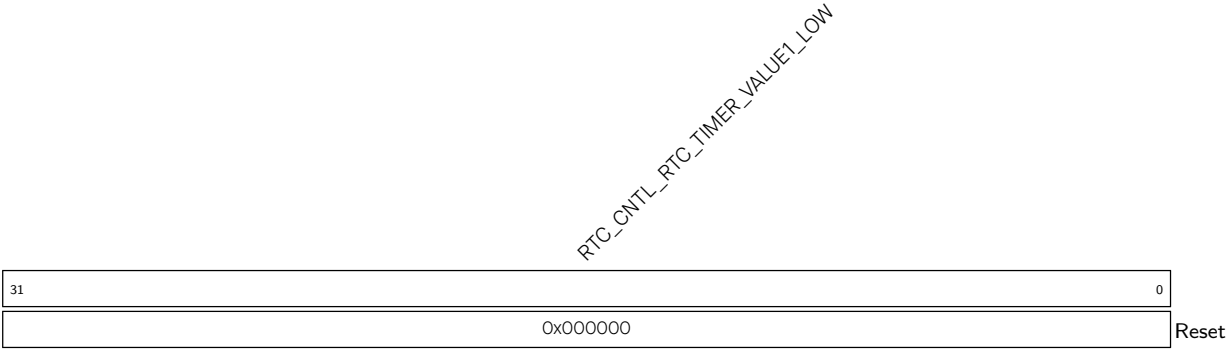
Register 10.52. RTC_CNTL_RTC_TIME_LOW1_REG (0x00EC)
