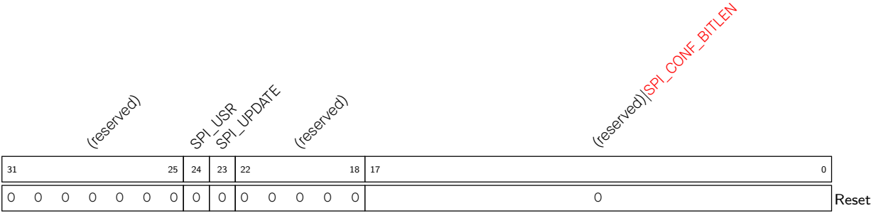
Register 30.1. SPI_CMD_REG (0x0000)
