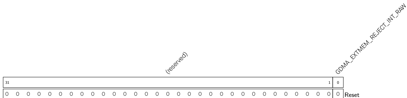
Register 3.19. GDMA_EXTMEM_REJECT_INT_RAW_REG (0x03FC)
