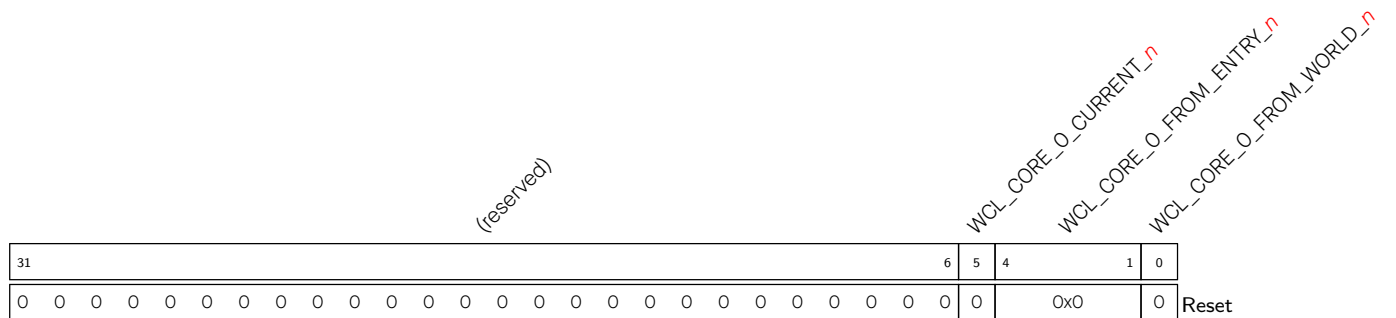
Register 16.6. WCL_CORE_O_STATUSTABLE n _REG ( n : 1-13) (0x0080+4*( n -1))
