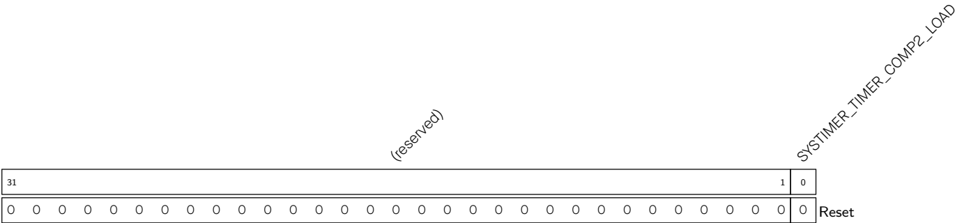
Register 11.25. SYSTIMER_COMP2_LOAD_REG (0x0058)
