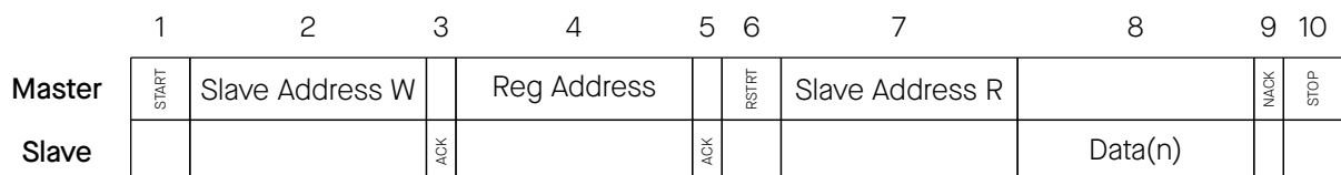
Figure 2.7-1. I2C Read Operation
