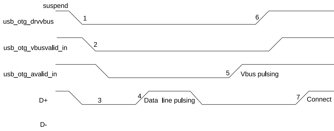
Figure 32.4-1. A-Device SRP
