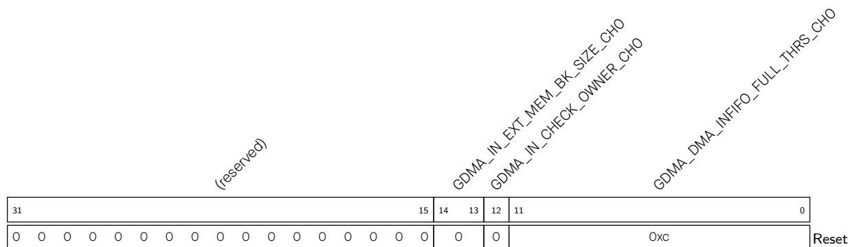
Register 3.2. GDMA_IN_CONF1_CH n _REG ( n : 0-4) (0x0004+192* n )
