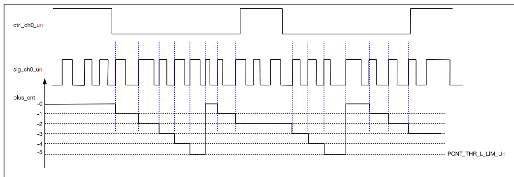
Figure 38.3-2. Channel 0 Down Counting Diagram
