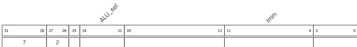
Figure 2.5-4. Instruction Type — ALU for Operations with Stage Count Register
