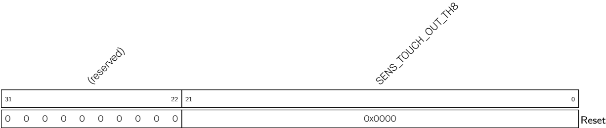
Register 39.29. SENS_SAR_TOUCH_THRES8_REG (0x0080)
