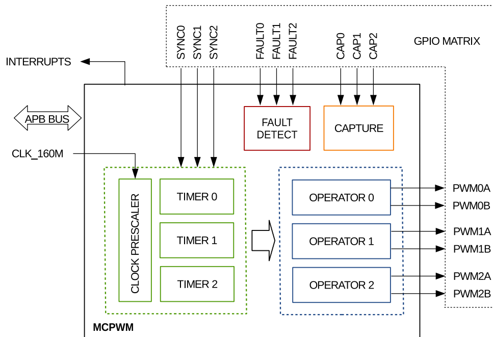
Figure 36.2-1. MCPWM Module Overview
