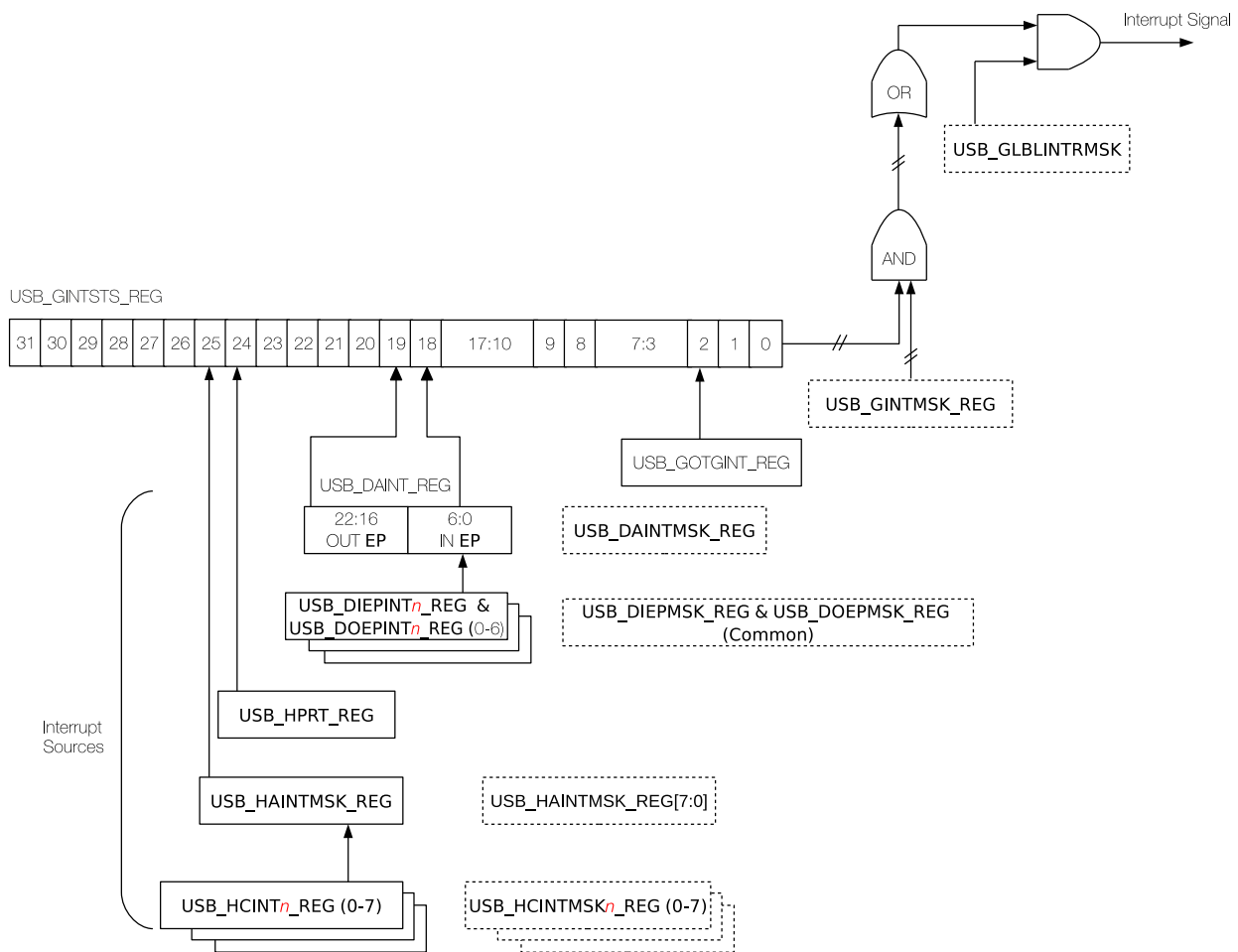
Figure 32.3-5. OTG_FS Interrupt Hierarchy
