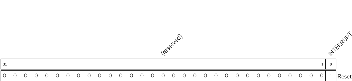
Register 9.179. INTERRUPT_CORE1_CLOCK_GATE_REG (0x099C)
