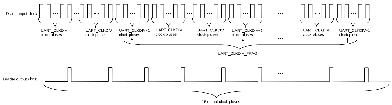
Figure 26.4-2. UART Controllers Division
