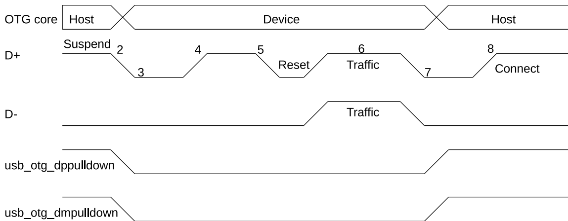
Figure 32.4-3. A-Device HNP
