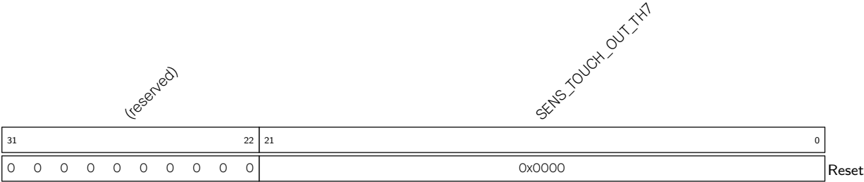
Register 39.28. SENS_SAR_TOUCH_THRES7_REG (0x007C)
