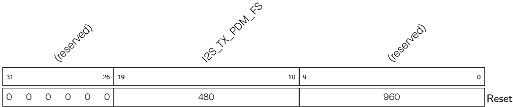
Register 28.9. I2S_TX_PCM2PDM_CONF1_REG (For I2S0 Only) (0x0044)
