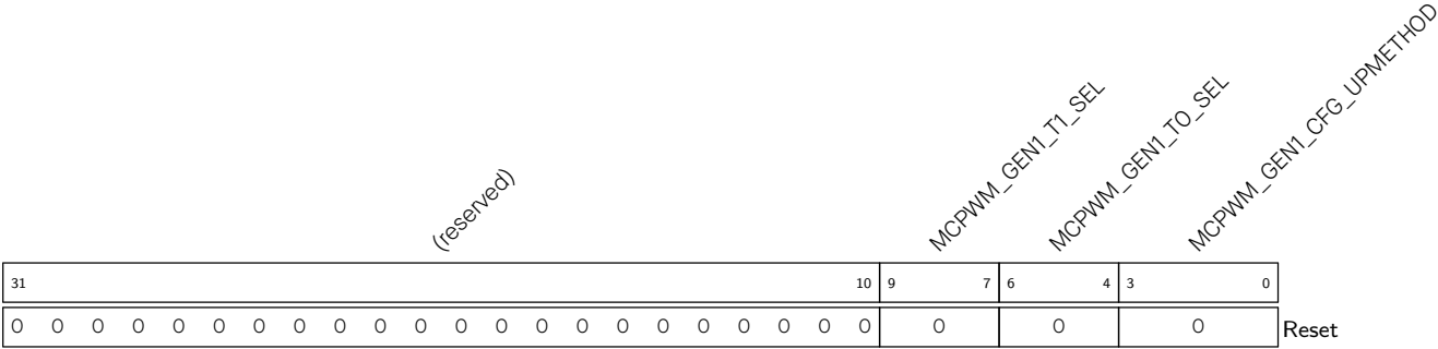
Register 36.33. MCPWM_GEN1_CFG0_REG (0x0080)
