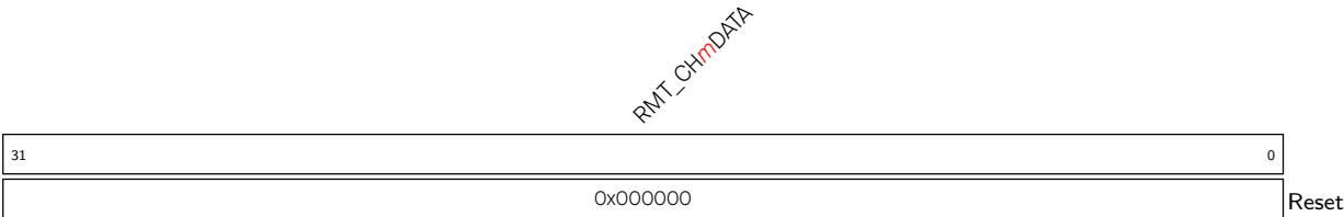
Register 37.2. RMT_CHmDATA_REG (m = 4, 5, 6, 7) (0x0010, 0x0014, 0x0018, 0x001C )
