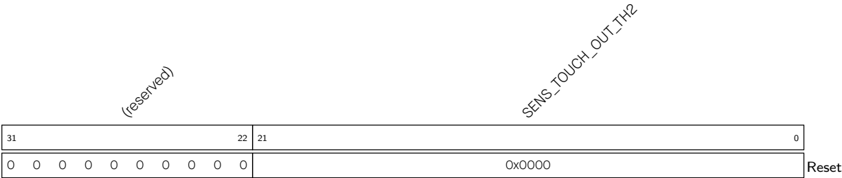
Register 39.23. SENS_SAR_TOUCH_THRES2_REG (0x0068)
