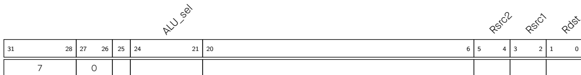
Figure 2.5-2. Instruction Type — ALU for Operations Among Registers
