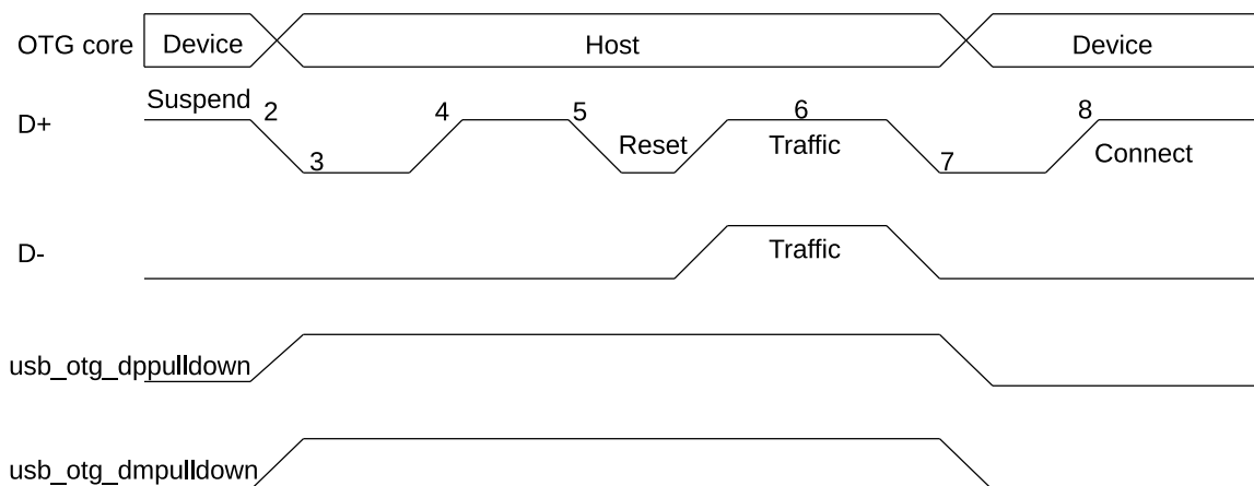
Figure 32.4-4. B-Device HNP
