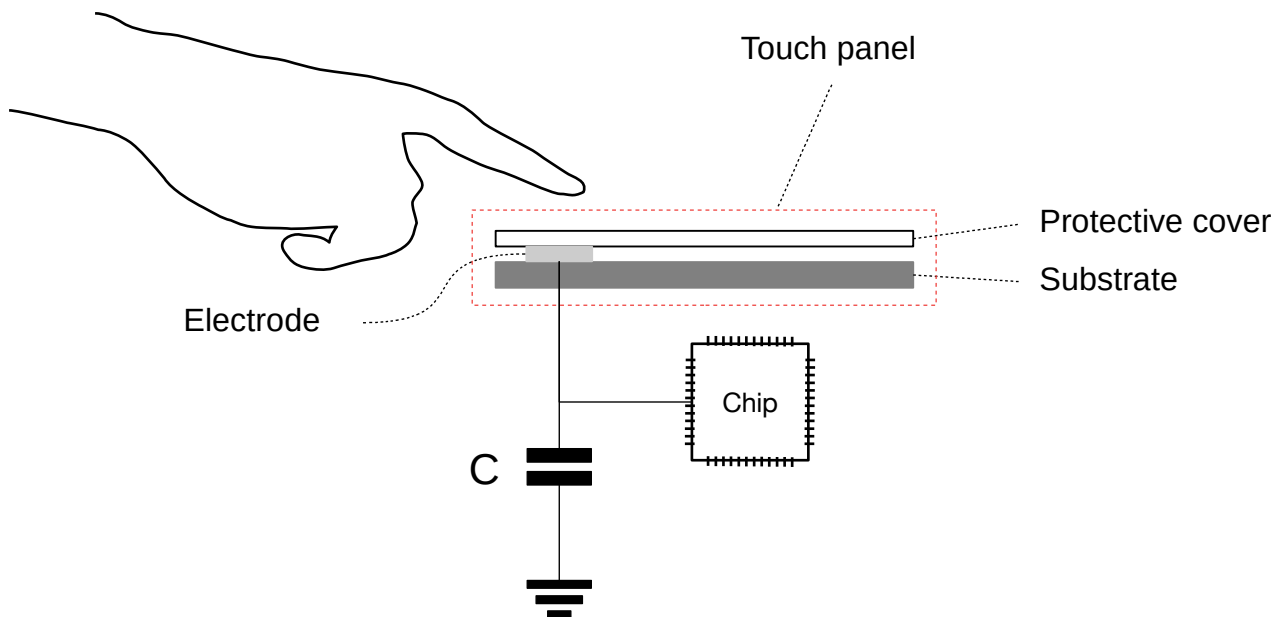
Figure 39.2-1. Touch Sensor
