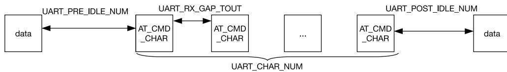
Figure 26.4-5. AT_CMD Character Structure
