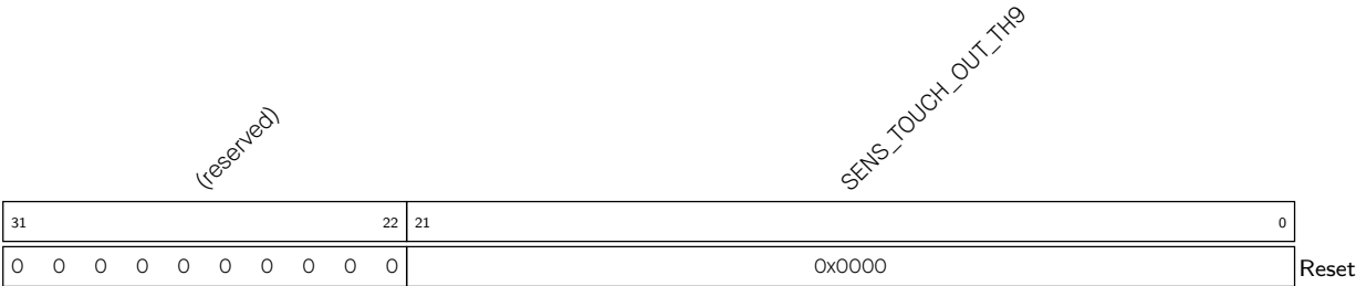
Register 39.30. SENS_SAR_TOUCH_THRES9_REG (0x0084)
