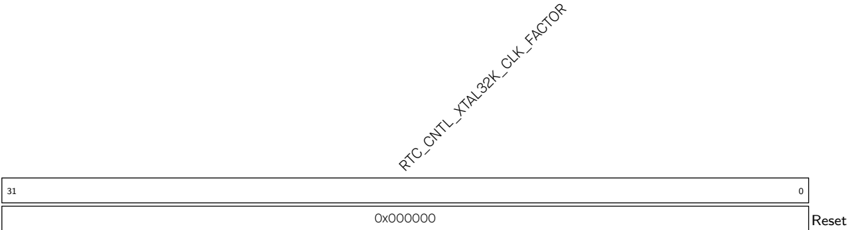
Register 10.54. RTC_CNTL_RTC_XTAL32K_CLK_FACTOR_REG (0x00F4)
