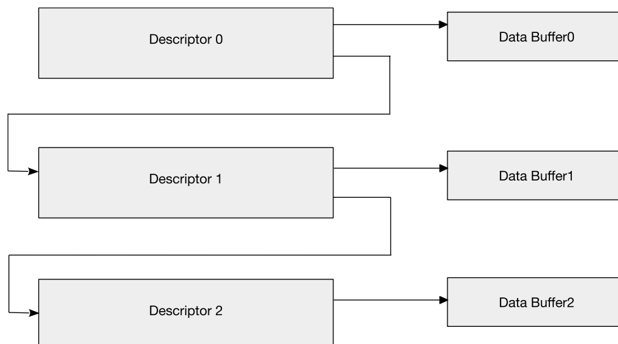
Figure 34.7-1. Descriptor Chain
