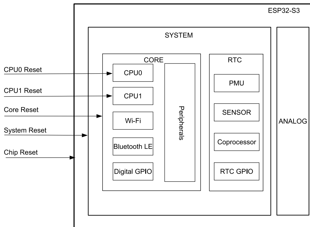
Figure 7.1-1. Reset Levels
