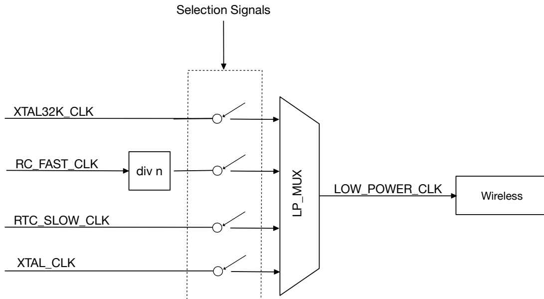
Figure 10.3-4. Wireless Clocks
