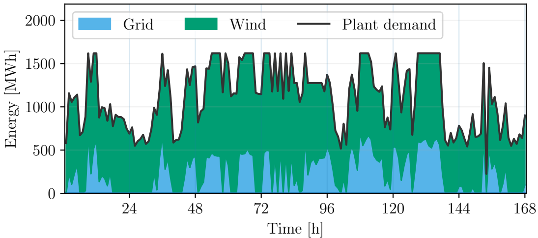
(c) Scenario 3
