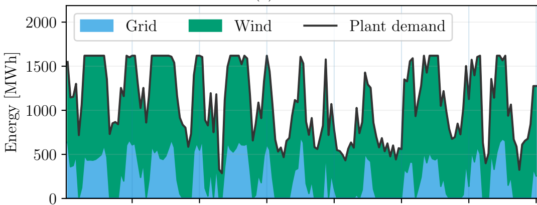
(a) Scenario 1
