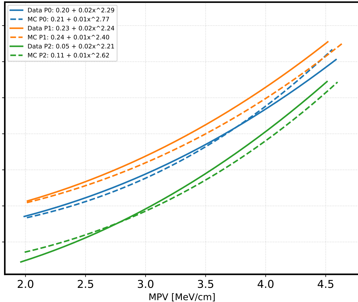
Pion Smearing: X > 0 (TPC 1)
