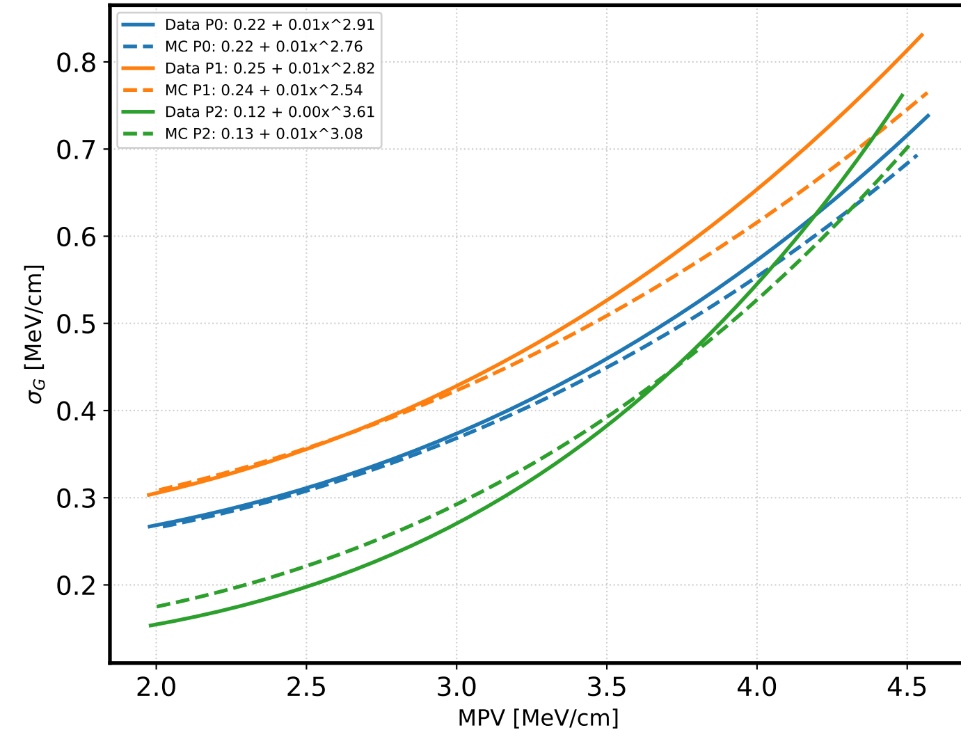
Pion Smearing: X < 0 (TPC 0)
