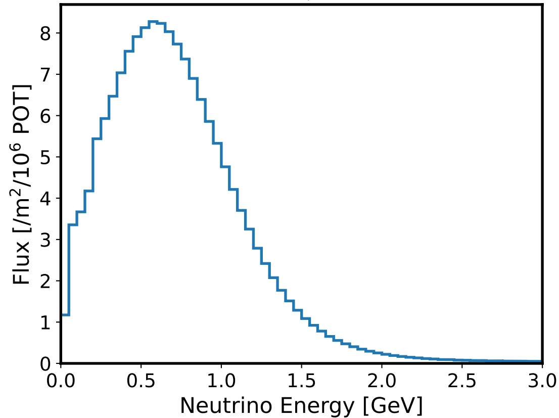
SBND \nu_\mu Flux
