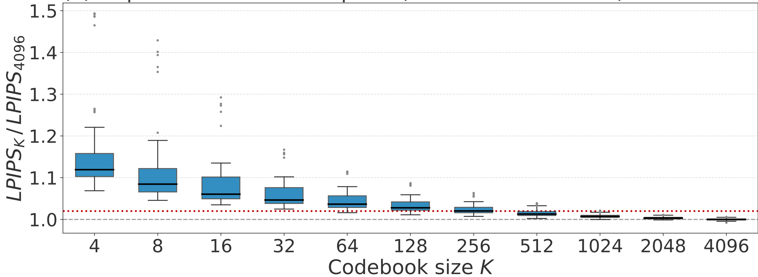
(b) dispersion over 65 runs per K (13 scenes \times 5 seeds)
