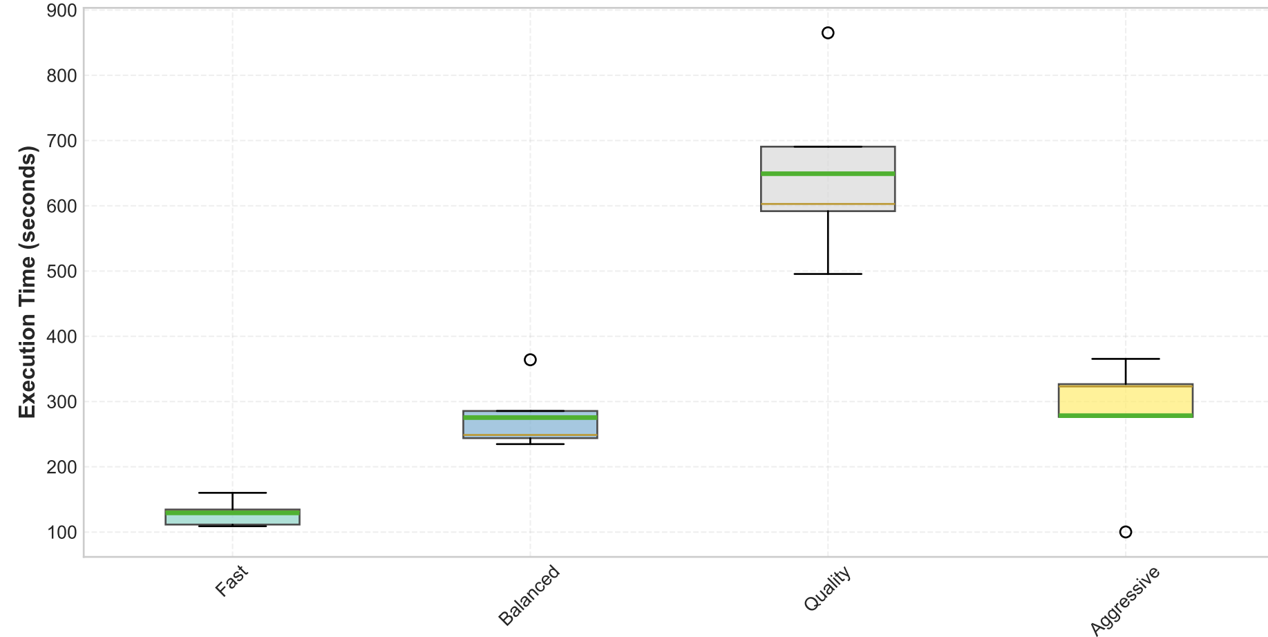
COMPUTATIONAL TIME DISTRIBUTION BY CONFIGURATION
