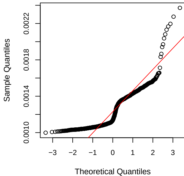
Q-Q Go gRPC - Payload 50000
