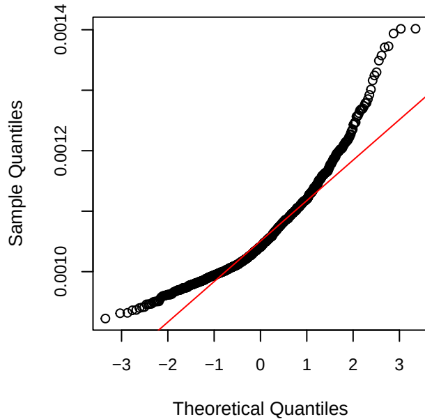
Q-Q Go gRPC – Payload 5000
