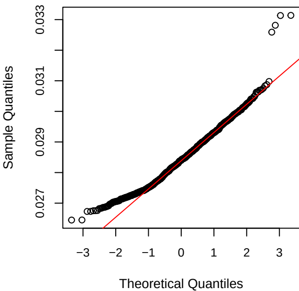
Q-Q Go REST – Payload 150000
