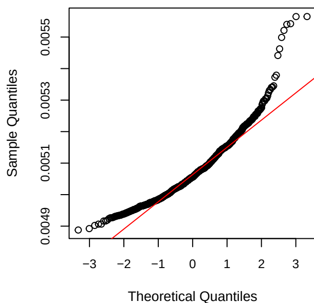
Q-Q Go gRPC – Payload 204800
