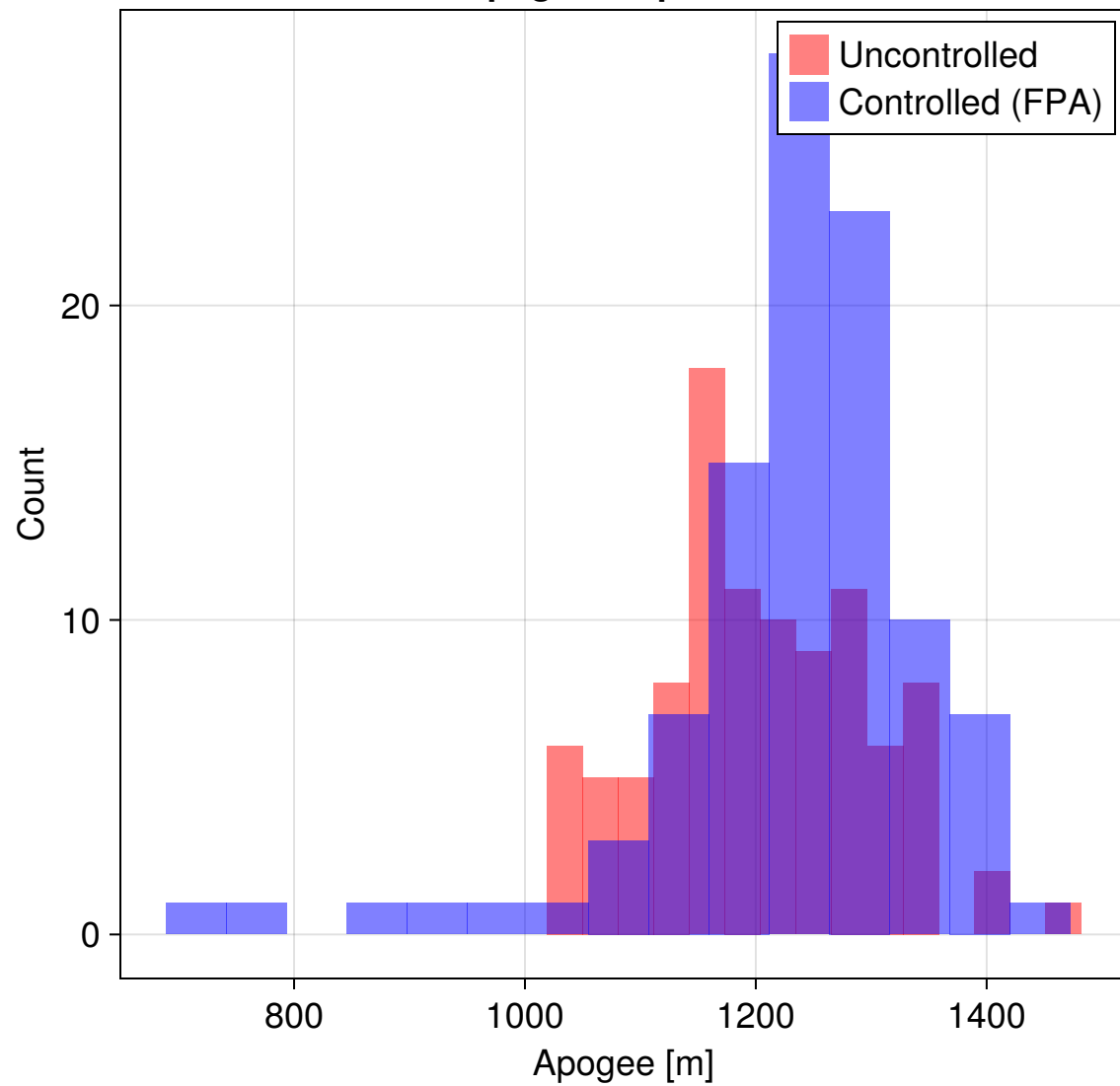
Apogee Dispersion
