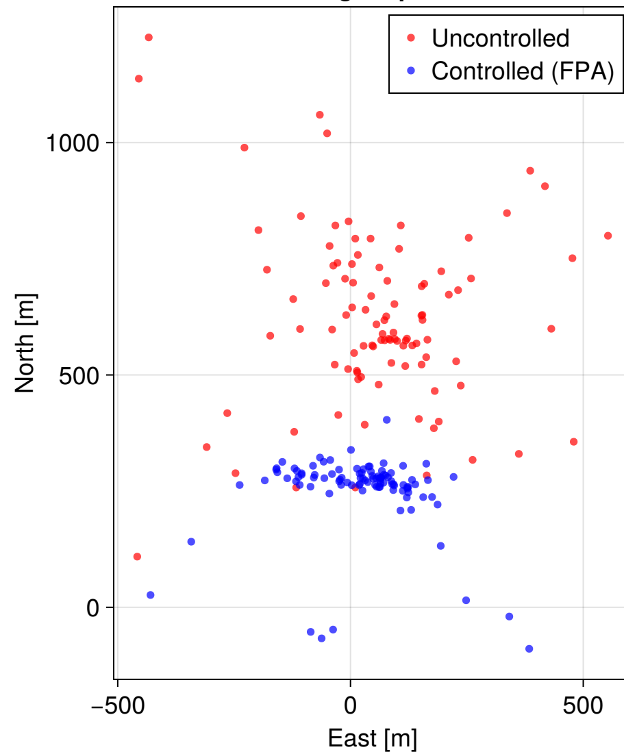
Landing Dispersion
