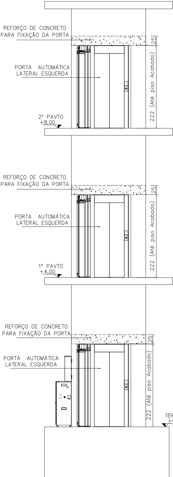
VISTA FRONTAL
