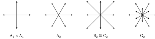
Rank 2 root systems.
