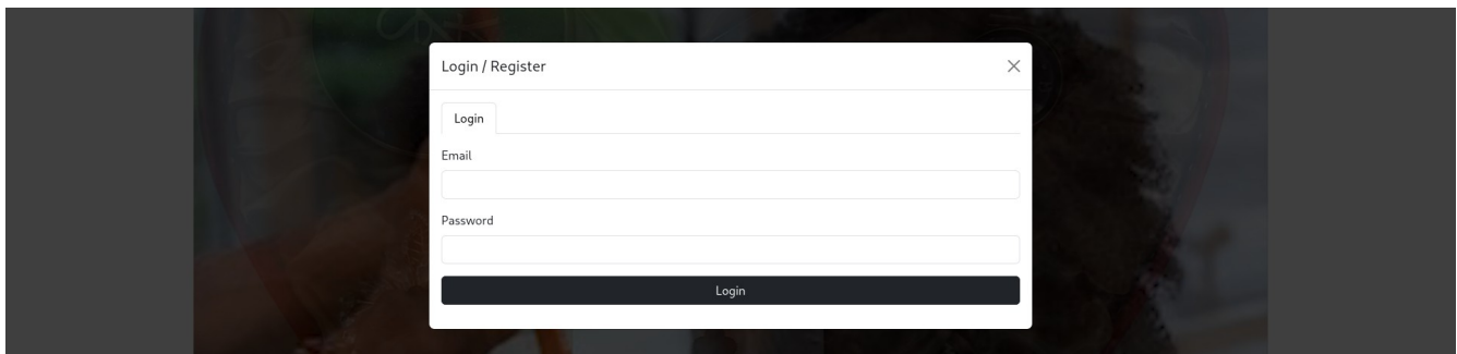
Figure 1: Login Form
