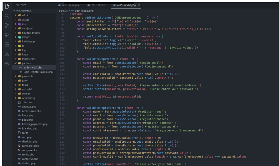
Figure 3: Folder Structure
