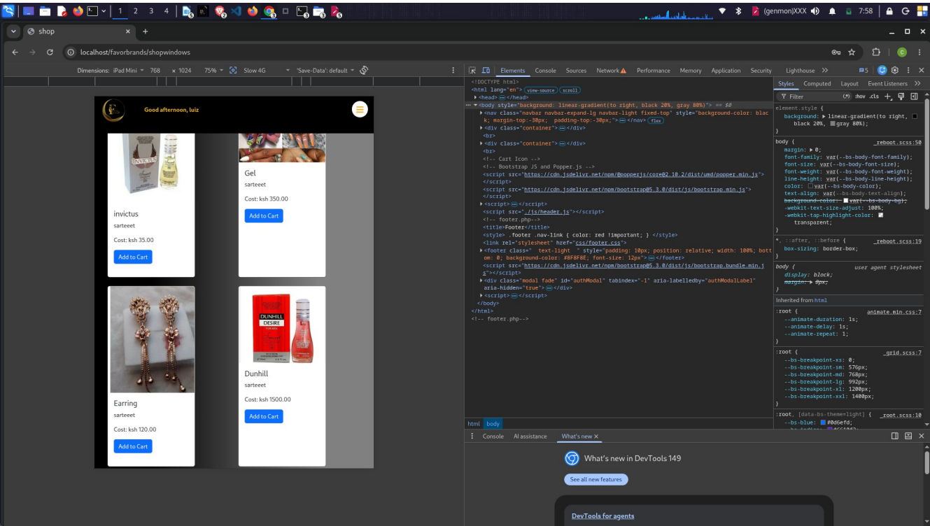
Figure 8.2: Tablet-View
