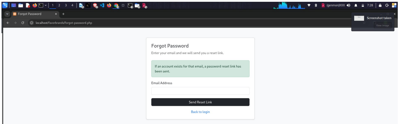
Figure 7.4: Reset-Password-Flow
