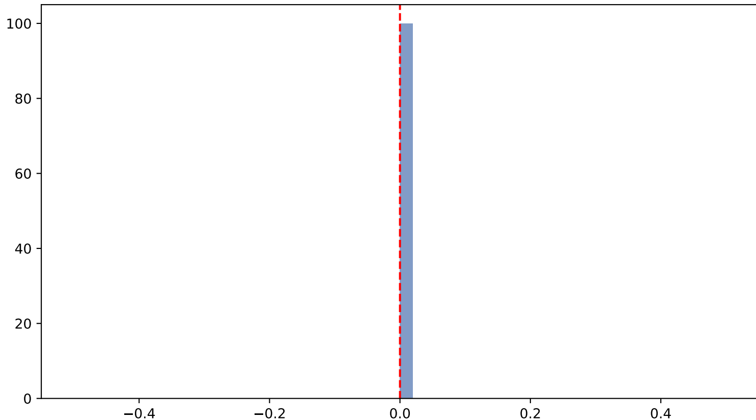
Permutation test (net_profit) p-value=1.0000
