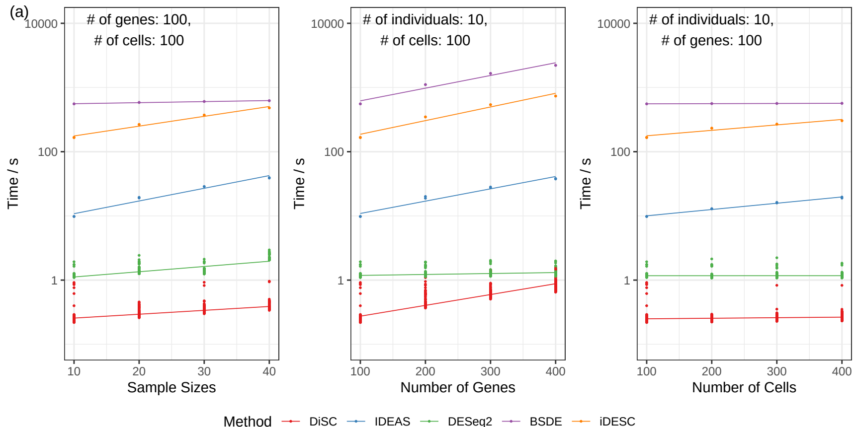
Computation Time (in Seconds) for Different Differential Expression Analysis Methods
