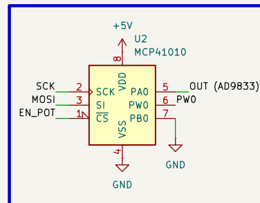
DIGITAL POTENTIOMETER
