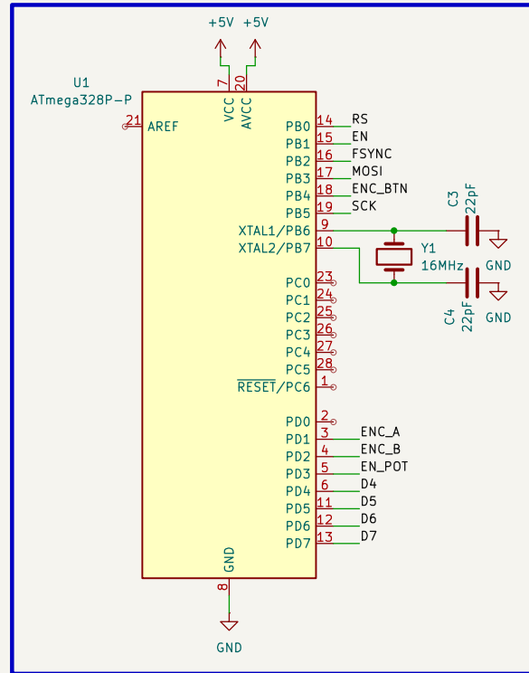
MICROCONTROLLER WITH CRYSTAL
