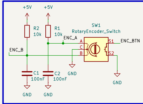
ROTARY ENCODER WITH SWITCH
