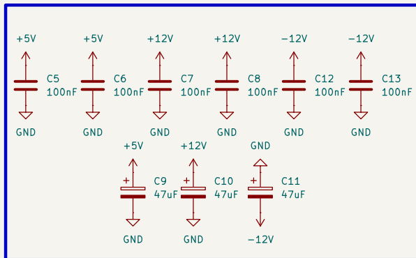
FILTERING CAPACITORS
