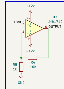
FINAL AMPLIFIER STAGE
