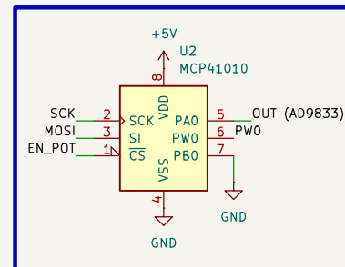
DIGITAL POTENTIOMETER
