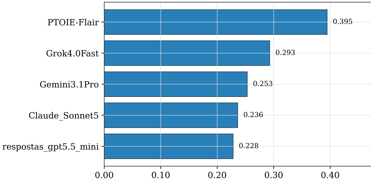
F1-Score (Lexical Match) — Respostas ExtrativoPTOIE-DP
