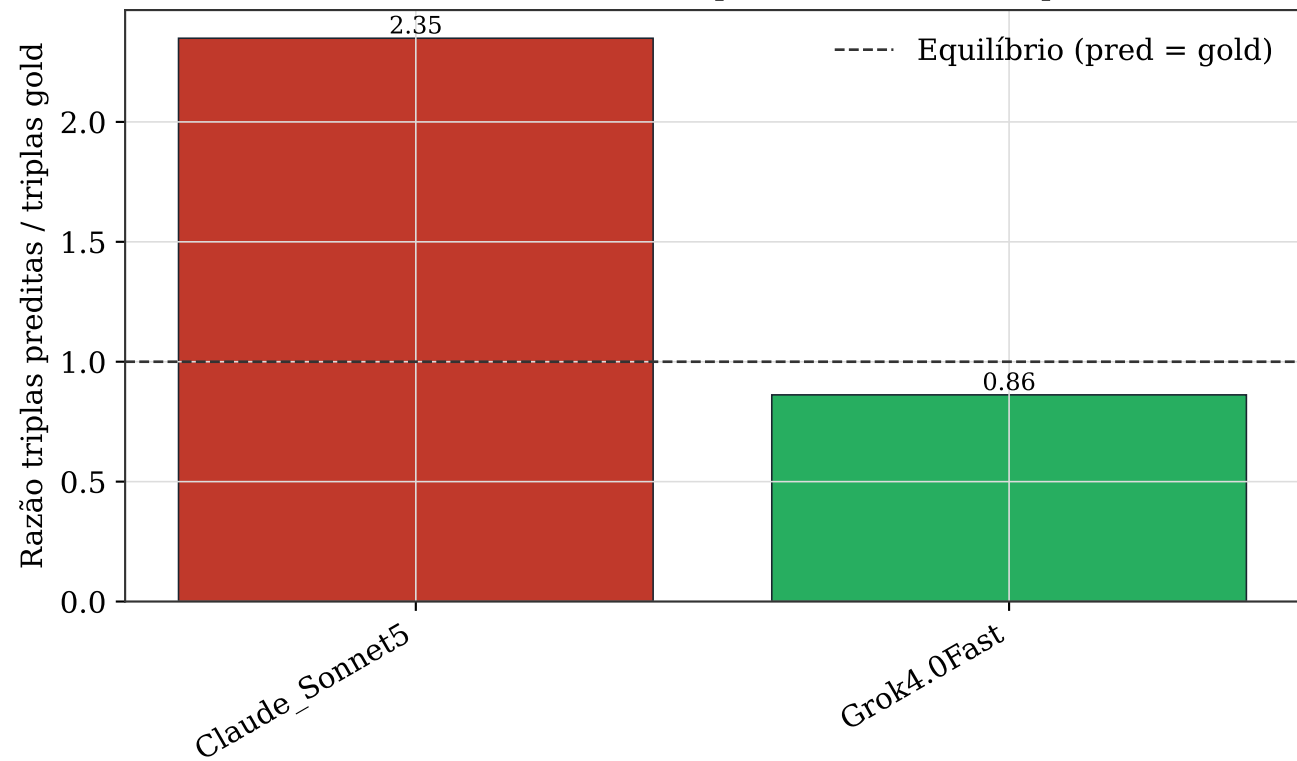
Razão Predito/Gold — Respostas AbstractiveOpenIE
