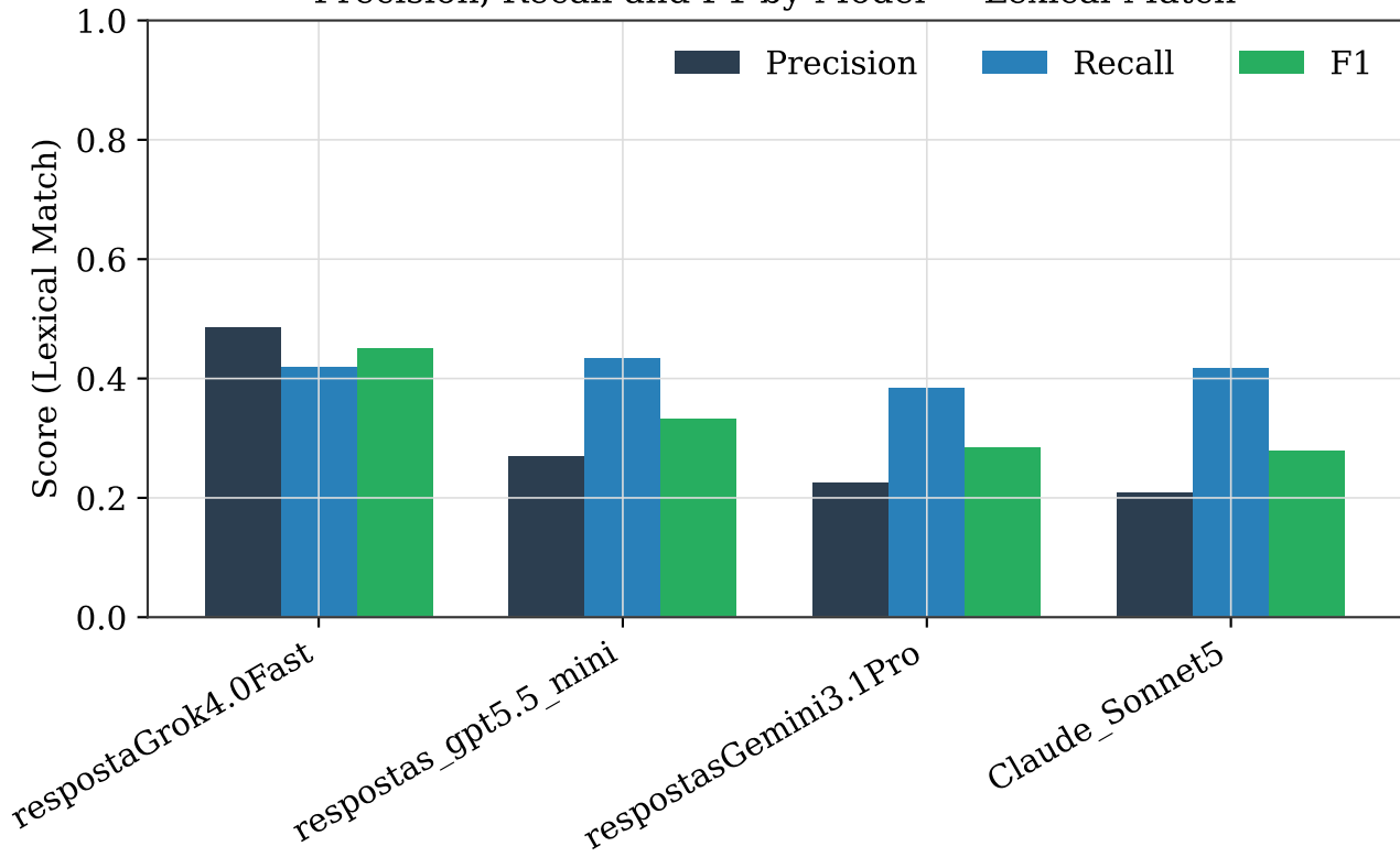
Precision, Recall and F1 by Model — Lexical Match
