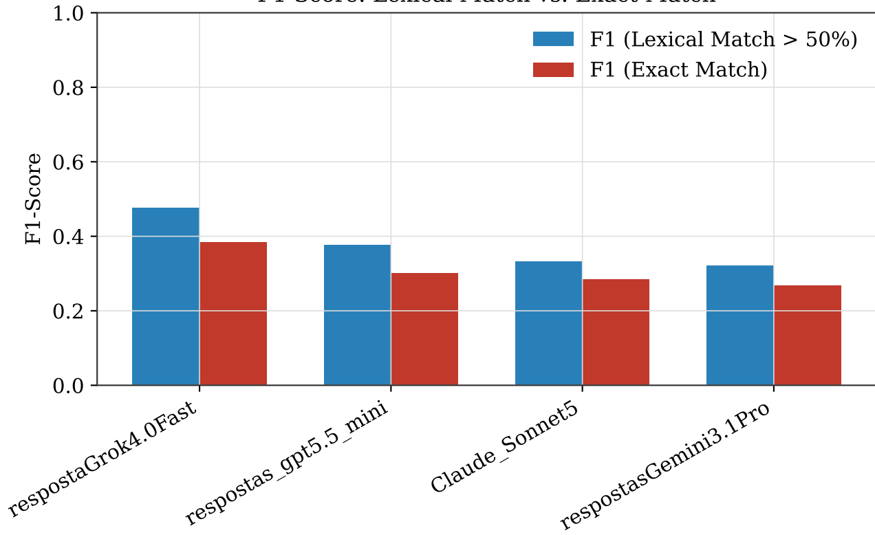
F1-Score: Lexical Match vs. Exact Match
