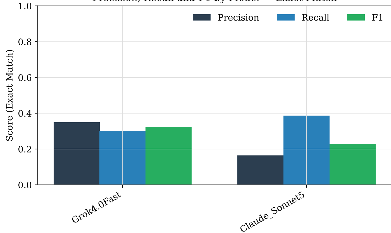
Precision, Recall and F1 by Model — Exact Match
